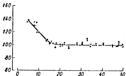
Intensity of photosynthesis in Closteriopsis acicularis according to carbon dioxide uptake (dots) and biomass increment (crosses) as a function of concentration of oxygen in atmosphere X-axis, oxygen concentration (%), y-axis, intensity of photosynthesis (%)
