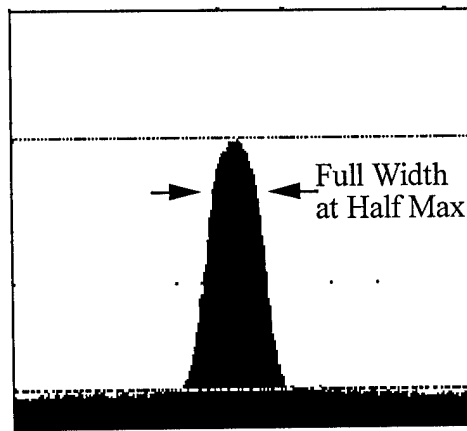
Sample Display of Line Width Measurement using Diode Optics on Monochrome Screen
