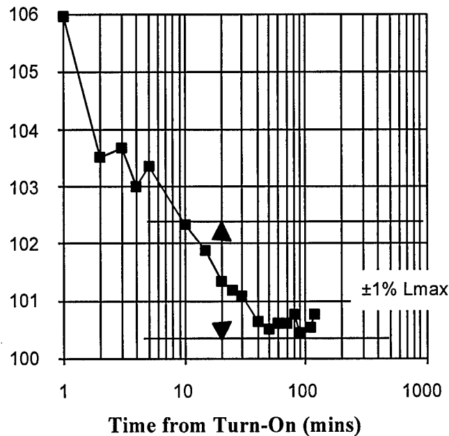
Plot of luminance as a function of time showing warmup characteristic.
