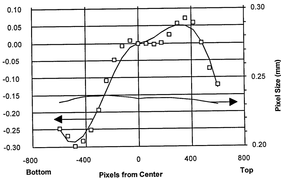
Sample vertical linearity characteristics. The open boxes are measured data fitted with a cubic equation, shown by the line. The derived pixel size is also shown.
