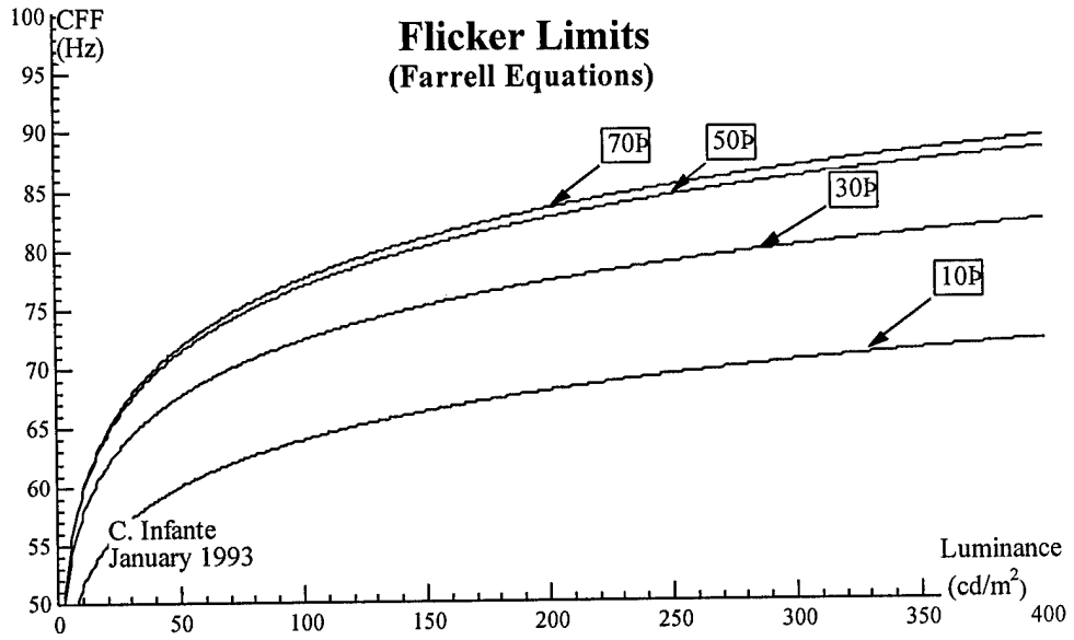
Plot of critical flicker frequency versus display luminance for various display sizes specified in degrees of visual angle.
