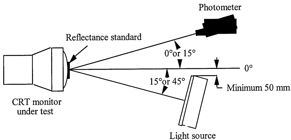
General test setup for reflectance measurement (from ISO 9241 part 7).
