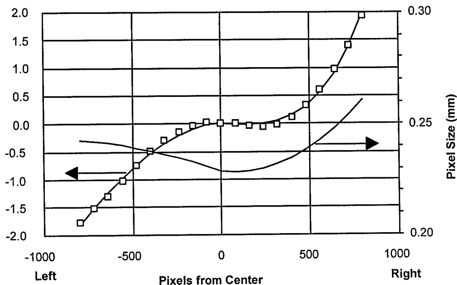
Sample horizontal linearity characteristics. The open boxes are measured data fitted with a cubic equation, shown by the line. The derived pixel size is also shown.
