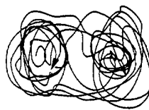
A chaotic orbit (in 3D or higher)
