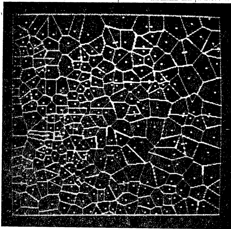
Figure 6. Voronoy's Polygons Constructed by VOPLES Program
