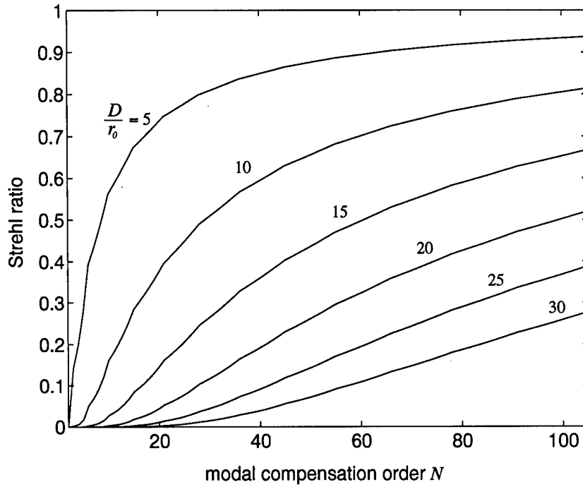
Figure 8. Effect of modal compensation order N on Strehl ratio for the relative aperture diameter D/r_0 .
