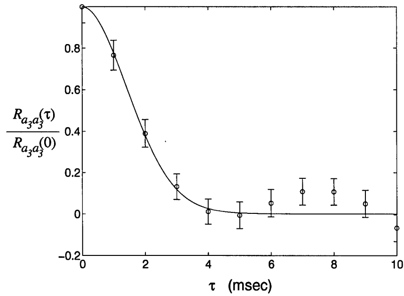
Figure 18. Comparison of theoretical and experimental temporal autocorrelation results for tilt components. (a) Temporal autocorrelation of the x-tilt (Zernike 2) and (b) temporal autocorrelation of the y-tilt (Zernike 3) for the reconstructed phase measurements studied. Experimental results are shown with error bars, and theoretical results are indicated by the solid curves.
