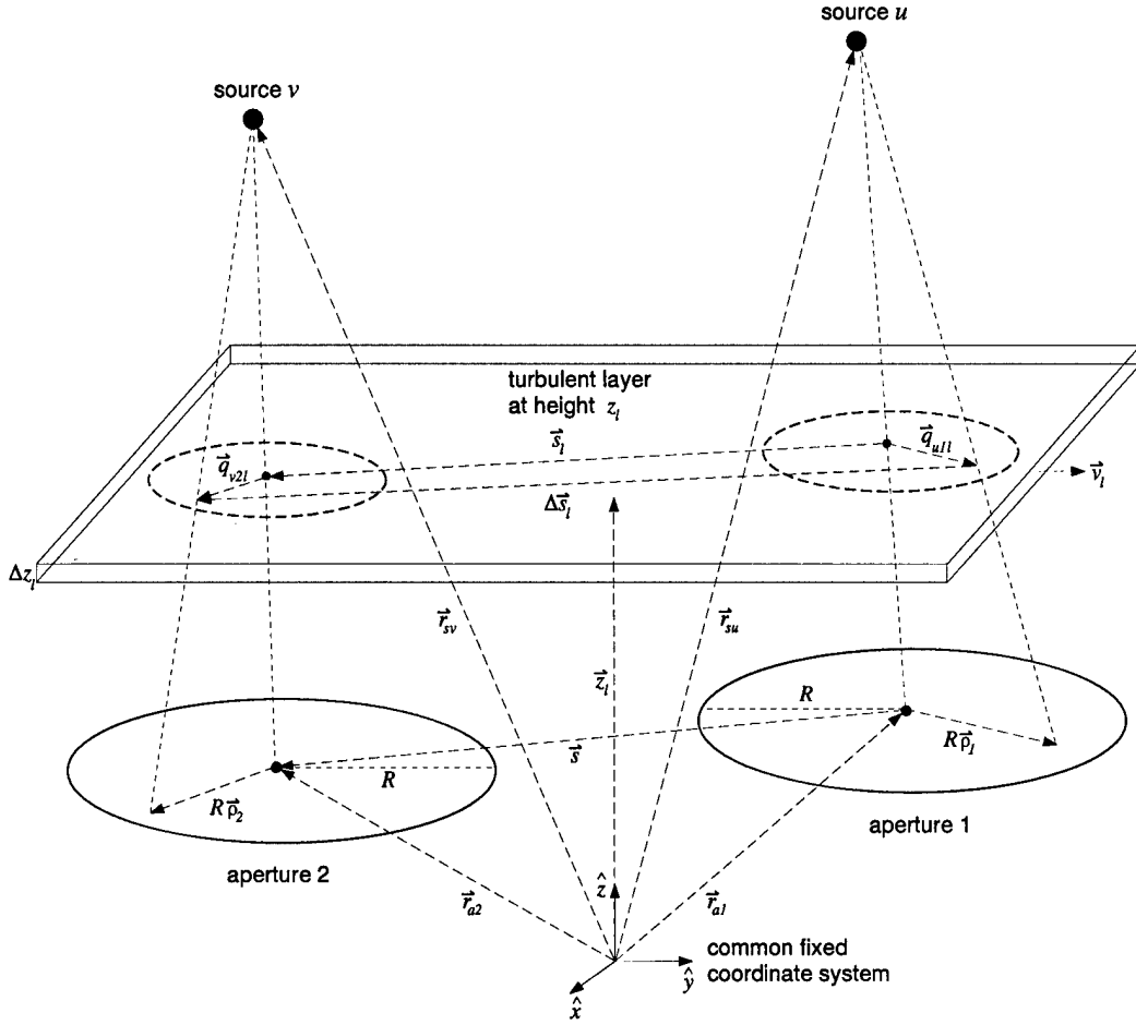
Figure 12. Analysis geometry used for computing the spatial cross-correlation of Zernike expansion coefficients.
