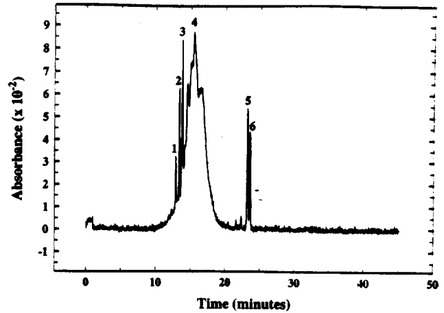
FIGURE 4 CZE electropherogram of rabbit tear protein derivatized with ATTO-TAG CBQ, performed using 50 mM borate running buffer, pH 8.5, at 11 kV and 23 °C, with LIF detection.
