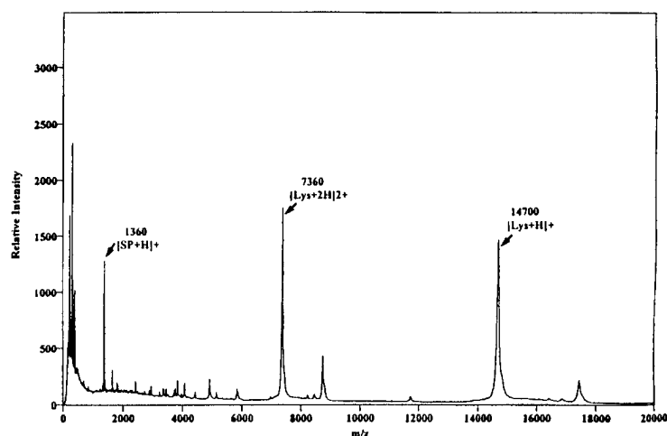
Figure 1. A MALDI mass spectrum of substance P ( m/z = 1360 ) naturally occurring in undiluted tears collected from a healthy 28-year-old man who did not wear contact lenses and who was asymptomatic for dry eye syndrome. Lys+H and Lys+2H are lysozyme and its doubly protonated form, respectively (2).
