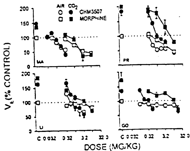
FIG. 7. Dose-effect curves for cumulative doses of morphine (squares) and OHM3507 (circles) on ventilation ( V_E ) in air (open symbols) and in 5% CO_2 (closed symbols) in four monkeys. Ordinate: averaged V_E expressed as a percentage of V_E under control conditions. Abscissa: dose in mg/kg of body weight. Points above C represent the measures of ventilation obtained under control (no drug) conditions.
