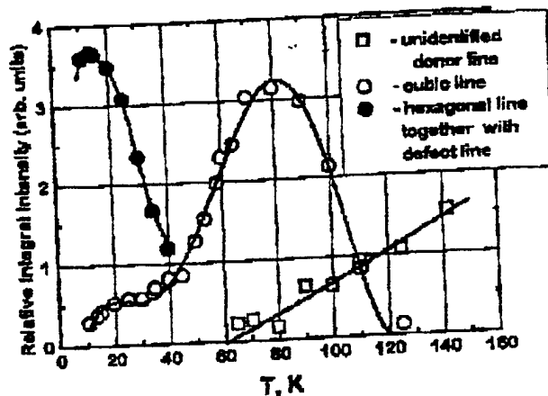
Fig.8. Temperature dependencies of the relative integral intensities of ESR spectra of 6H SiC irradiated with neutron beam (flux \Phi = 2 \cdot 10^{18} \text{ cm}^{-2} , T_{\text{ann}} = 1400^\circ\text{C} ). Concentration of uncompensated nitrogen ( N_D - N_A ) \approx 5 \cdot 10^{17} \text{ cm}^{-3} . \nu_{\text{ESR}} = 9 \text{ GHz} .
