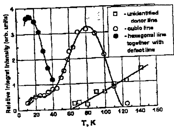
Fig. 8. Temperature dependencies of the relative integral intensities of ESR spectra of 6H SiC irradiated with neutron beam (flux \Phi = 2 \cdot 10^{18} \text{cm}^{-2} , T_{\text{ann.}} = 1400^\circ\text{C} ). Concentration of uncompensated nitrogen ( N_D - N_A ) \approx 5 \cdot 10^{17} \text{cm}^{-3} . \nu_{\text{ESR}} = 9 \text{ GHz} .
