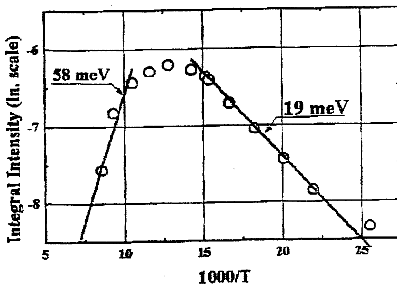
Fig. 5. Temperature dependencies of the integral intensities of ESR spectra of nitrogen in cubic sites in bulk 6H SiC with (N_D - N_A) \approx 3 \cdot 10^{17} \text{cm}^{-3} . The solid lines are fitted by \exp(\Delta/kT) with \Delta = 58 \text{ meV} and 19 \text{ meV} .
