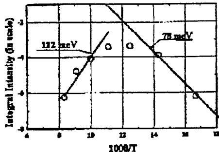
Fig.12. Temperature dependencies of the integral intensities of ESR spectra of nitrogen in cubic sites in 6H SiC EL with uncompensated nitrogen concentration of (N_D - N_A) \approx 7 \cdot 10^{16} \text{ cm}^{-3} . The solid lines are fitted by \exp(\Delta/kT) with \Delta = 112 \text{ meV} and 78 \text{ meV} .
