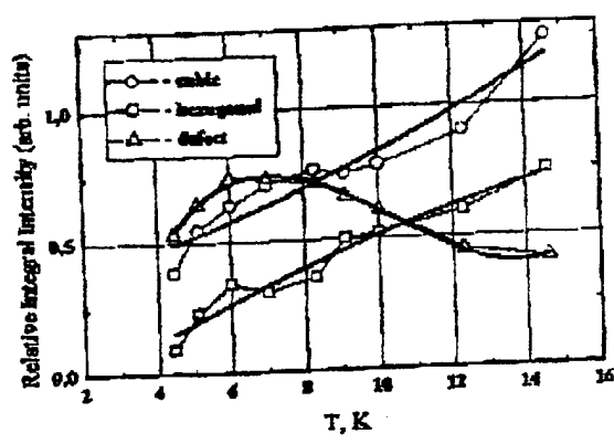
Fig. 9. Temperature dependencies of the relative integral intensities of ESR spectra of 6H SiC irradiated with neutron beam (flux \Phi = 2 \cdot 10^{18} \text{cm}^{-2} , T_{\text{ann.}} = 1400^\circ\text{C} ). Concentration of uncompensated nitrogen ( N_D - N_A ) \approx 5 \cdot 10^{17} \text{cm}^{-3} . \nu_{\text{ESR}} = 140 \text{ GHz} .
