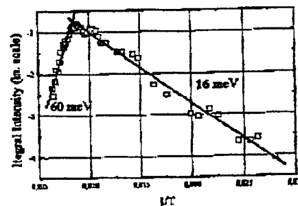
Fig. 3. Temperature dependencies of the integral intensities of ESR spectra of nonlocalized nitrogen electrons in bulk 6H SiC with (N_D - N_A) \approx 2 \cdot 10^{18} \text{ cm}^{-3} . The solid lines are fitted by \exp(\Delta/kT) with \Delta = 60 \text{ meV} and 16 \text{ meV} .
