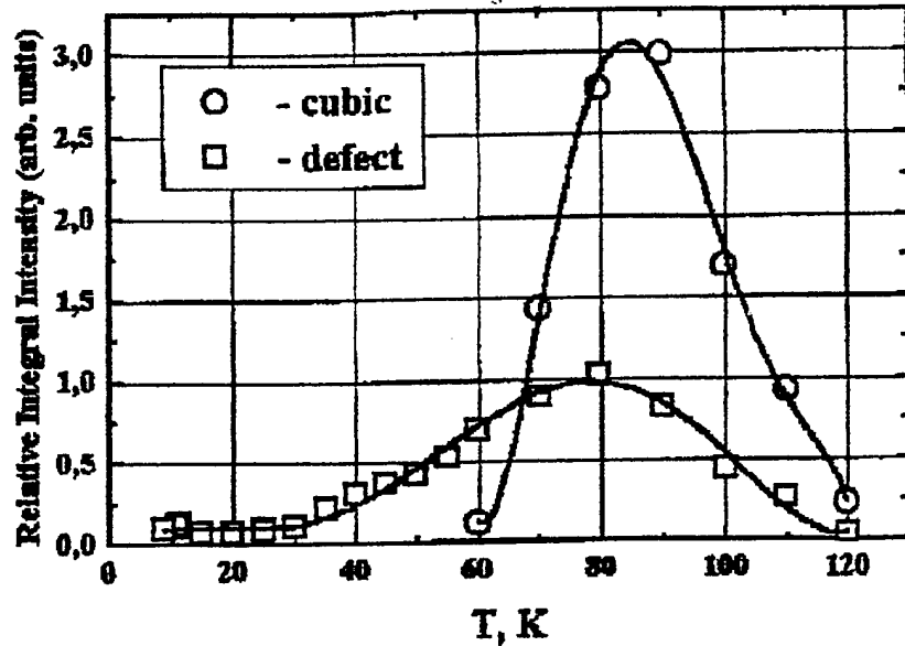
Fig.11 Temperature dependencies of the relative integral intensities of ESR spectra of 6H SiC EL with uncompensated nitrogen concentration of (N_D - N_A) \approx 7 \cdot 10^{16} \text{ cm}^{-3} .
