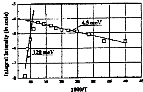
Fig.13. Temperature dependencies of the integral intensities of ESR spectra of nonidentified defect center in 6H SiC EL with uncompensated nitrogen concentration of (N_D - N_A) \approx 7 \cdot 10^{18} \text{ cm}^{-3} . The solid lines are fitted by \exp(\Delta/kT) with \Delta = 120 \text{ meV} and 4.5 \text{ meV} .
