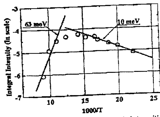
Fig. 10. Temperature dependencies of the integral intensities of ESR spectra of nitrogen in cubic sites in 6H SiC irradiated with neutron beam (flux \Phi = 2 \cdot 10^{18} \text{cm}^{-2} , T_{\text{ann.}} = 1400^\circ\text{C} ). Concentration of uncompensated nitrogen ( N_D - N_A ) \approx 5 \cdot 10^{17} \text{cm}^{-3} . The solid lines are fitted by \exp(\Delta/kT) with \Delta = 63 \text{ meV} and 10 \text{ meV} .
