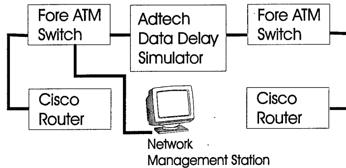
Figure 3: Lab Setup
