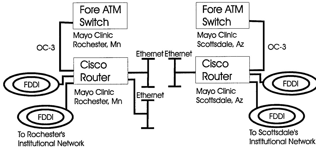
Figure 2: Legacy LAN
