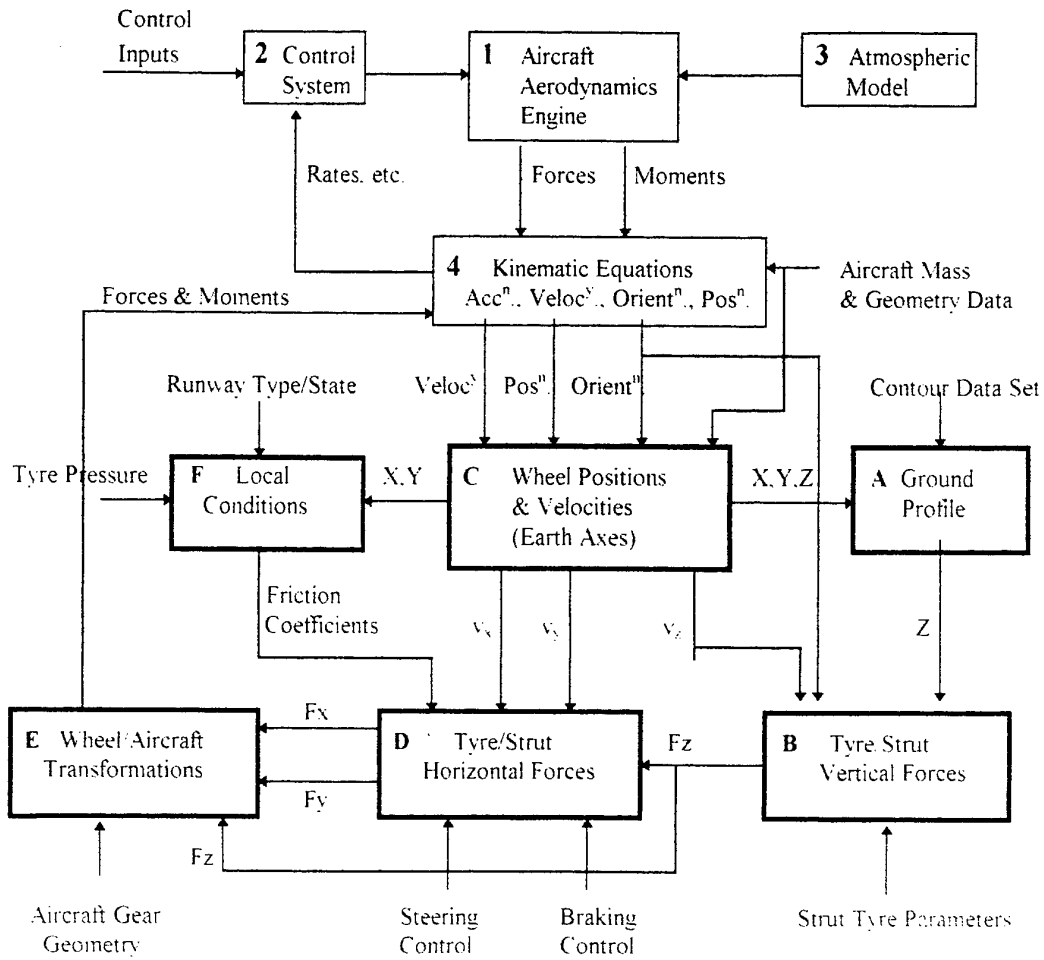
Figure 6.2 Structural model for ground roll simulation
