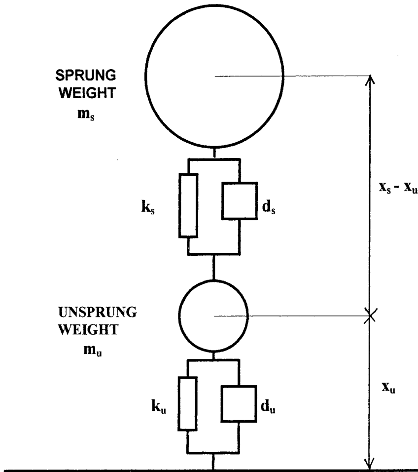
Figure A.1.2 Strut/wheel Equivalent Model
