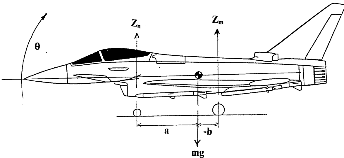
Figure A.1.3 Bounce/pitch modes
