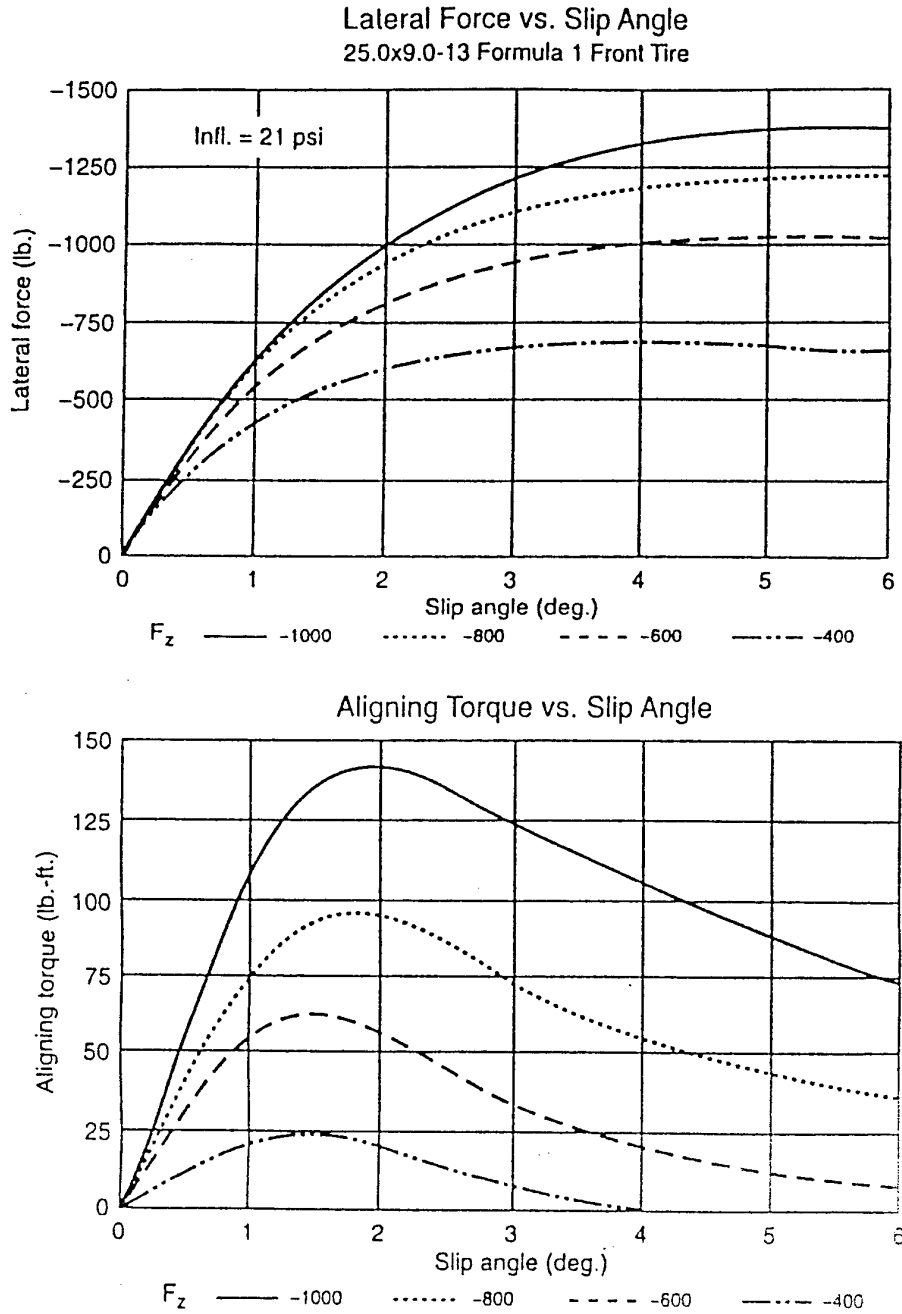
Figure 3.4 Lateral force and aligning torque v slip angle
