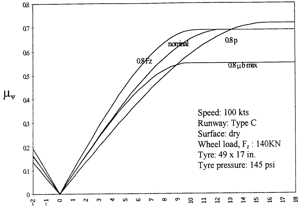
Figure A.3.1 Lateral friction coefficient v tire yaw angle
