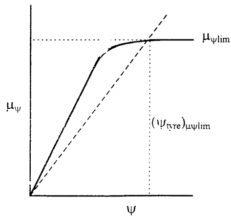
Figure A.3.2 Approximation for \mu_{\psi \text{ lim}} v \psi
