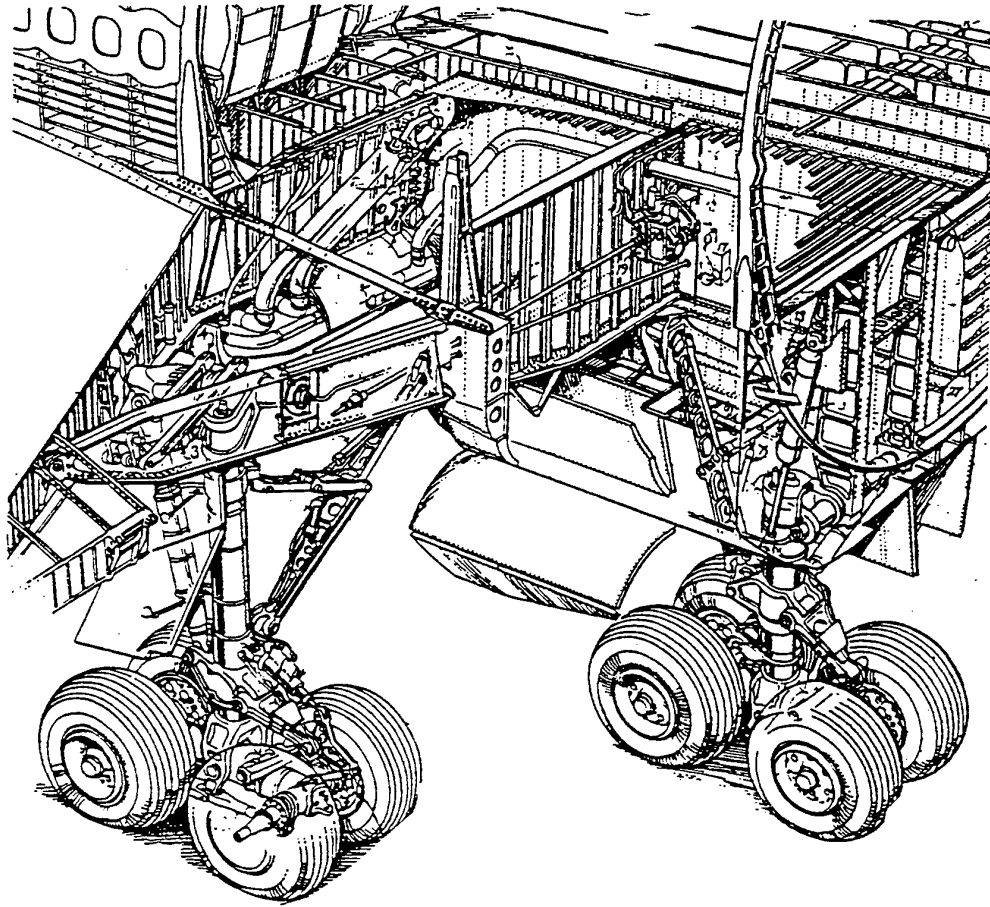
Figure 3.1 Boeing 747 main gear (port)
