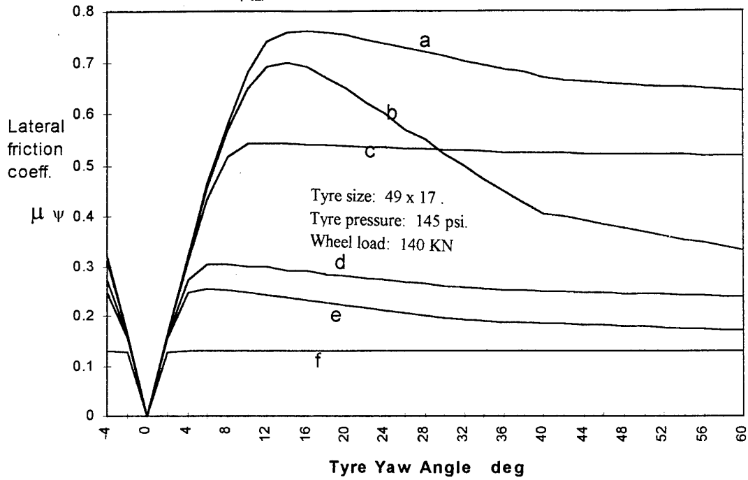
Figure A.3.6 Lateral friction coefficient v tire yaw angle
