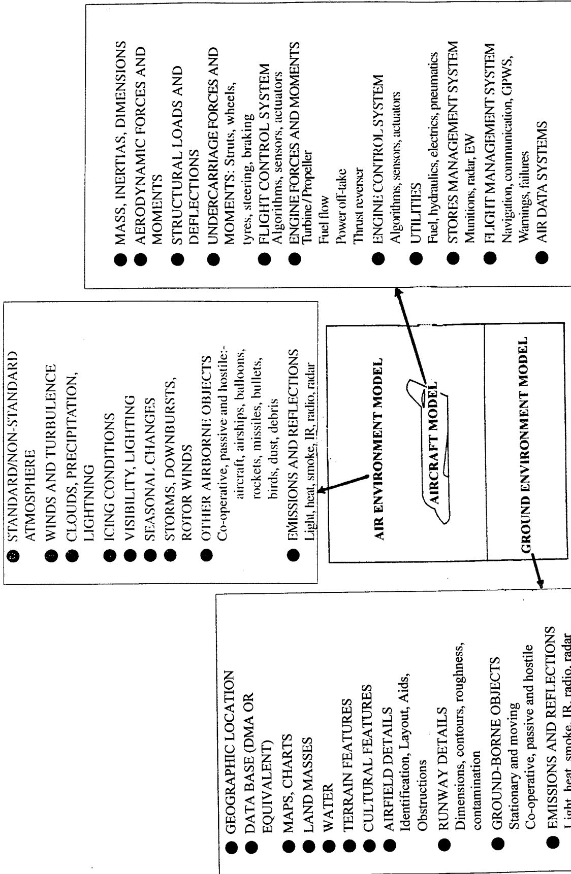
Figure 2.1 Model elements for flight simulation
