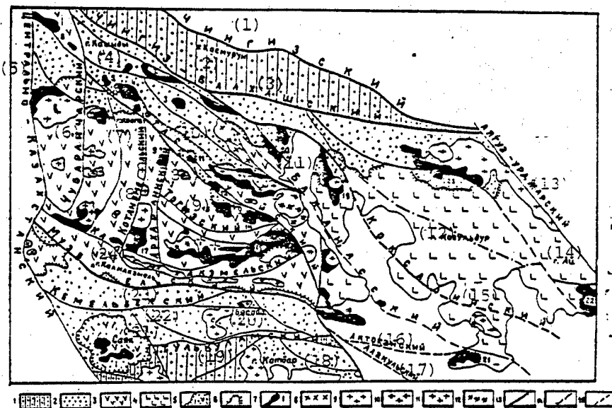
Diagram Showing Location of Intrusive Mountain Masses of the Northeastern Balkhash Region: 1-2--rock mass outcroppings of the lower structural stage, (E 1 -O-S-II-C 1 ); 3-5--rock mass outcroppings of the upper (orogenic) structural stage; 5--Kalamkamel'skaya zone, 4--Bakanasskaya zone, 5--Sayak'skaya zone; 6--boundary of the upper volcanogenic structural stage; 7--intrusive outcroppings of the Late Carbonaceous complex; 8--intrusive outcroppings of the Early Carbonaceous [continued on following page]
