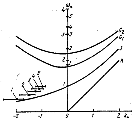
Figure 6. Dispersion diagram of equatorial waves. G_{1,2} --first and second modes of inertial-gravitational waves; J--mixed, K--Kelvin, in the lower left-hand part--different types of Rossby waves. Points 1-5--experimental estimates.
