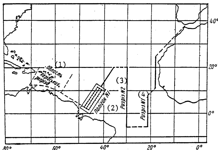
Figure 2. Diagram of patterns in tropical field test area.
