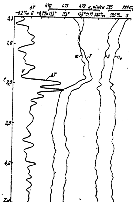
Figure 5. Microstructure of subsurface microthermocline in 0-5 m layer.
