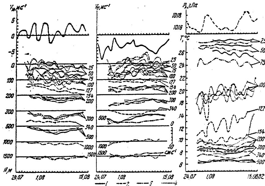
Figure 5. Change with time of the north-south V_m and zonal V_n components of current velocity and temperature T at various depths, measured by autonomous buoy stations (ABS). The upper part of the diagram shows the north-south and zonal components of wind velocity and atmospheric pressure P . The figures 1-4 indicate data obtained from different ABS.
