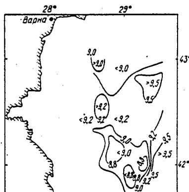
Figure 3. Horizontal distribution of temperature on the surface of Field Area 1.
