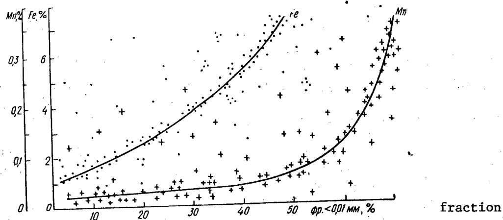
Fig. 1. Curves of dependence of concentration of iron and manganese on content of fraction < 0.01 mm in recent sediments of Ukrainian Black Sea shelf.
