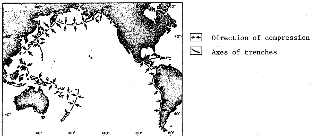
Map of orientation of compressions in lithosphere of inner (island and continental) slopes of Pacific Ocean trenches.
