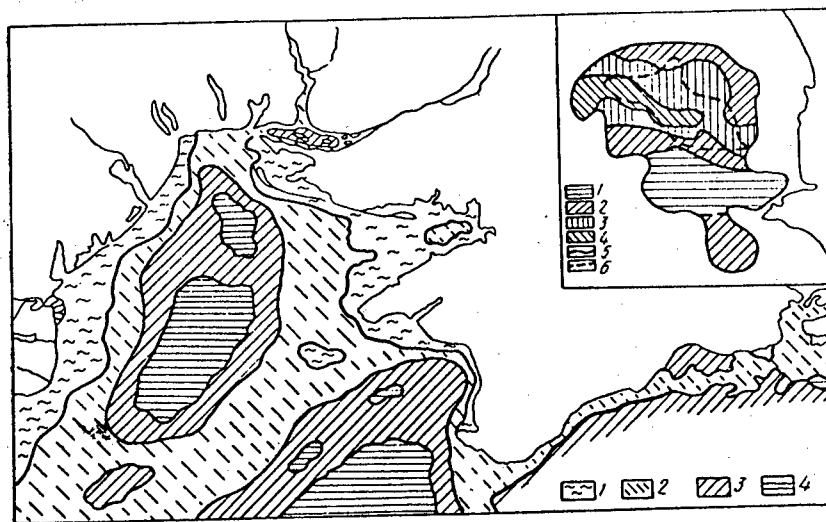
Fig. 2. Distribution of manganese in recent sediments on the Black Sea shelf of Ukrainian SSR (in % of noncalcareous matter of sediments): 1) less than 0.01; 2) 0.01-0.1; 3) 0.1-0.2; 4) more than 2.0%. In inset: Mn distribution in ferromanganese nodules of surface layer of Kalamitskoye field of nodules: 1) less than 2; 2) 2-6; 3) 6-10; 4) more than 10%; 5) limits of field of nodules; 6) limits of region with high content of nodules in sediments.
