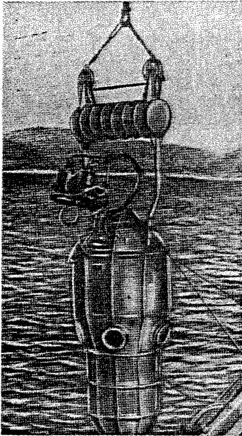
Fig. 1. "Sever-1" hydrostat.
