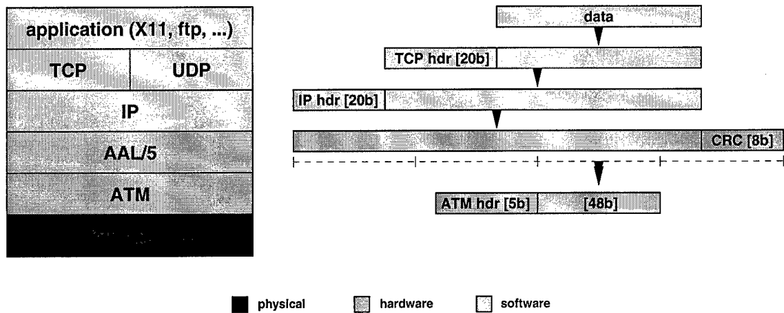
Figure 5: The protocol stack for our ATM-based TCP/IP network.
