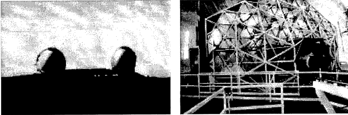
Figure 8: a. The domes of the twin 10-meter Keck Telescopes on Mauna Kea, Hawaii. b. The back of the primary mirror on the Keck I telescope, illustrating the network of 36 hexagonal segments which make up the mirror. The infrared camera is mounted at the forward Cassegrain focus of the telescope (i.e., in the central hole of the mirror).
