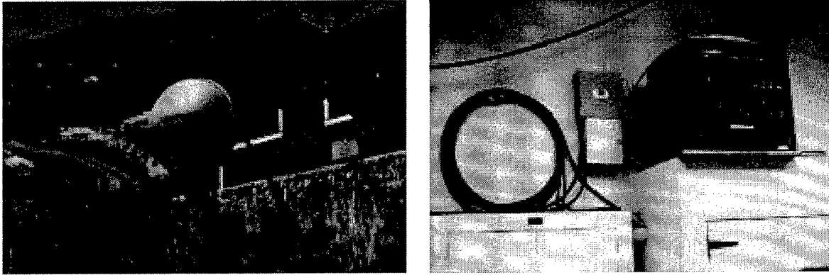
Figure 3: Hawaiian network infrastructure: a. A microwave relay station at Hale Pohaku, at the 9,000-foot level on Mauna Kea. Before the completion of a fiber network up the mountain in January of 1997, several dishes such as this one relayed data between Hale Pohaku and the base of the mountain. b. The ATM switch installed on the summit of Mauna Kea, in the Keck Telescope building. The switch is a Newbridge 36150 MainStreet ATMnet, provided by GTE Hawaiian Telephone. Two single-mode DS-3 cards are installed in the left end of the switch.
