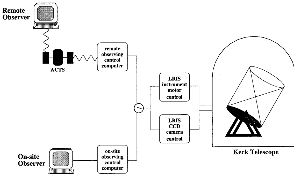
Figure 11: A schematic of the LRIS instrument control system at Keck Observatory. Note that there are two separate instrument control computers: one for standard on-site observations, and another for remote observations over the high-speed network.
