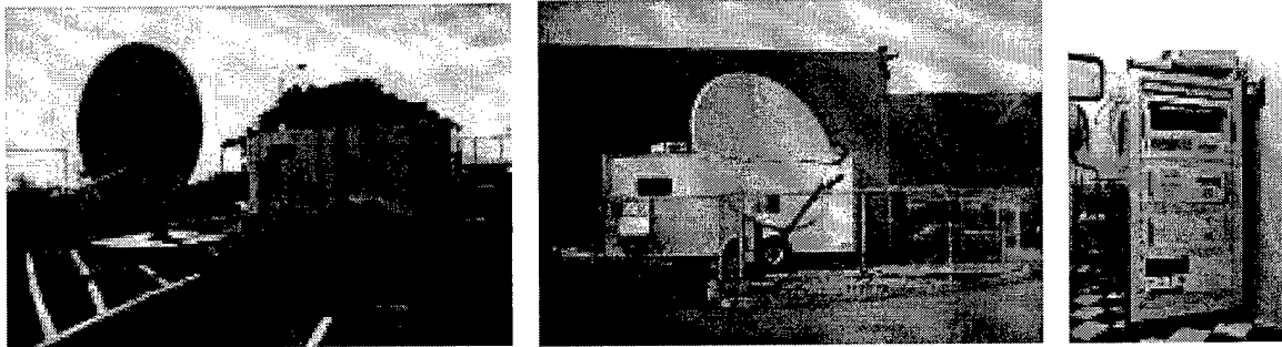
Figure 1: The ACTS high data rate (HDR) ground stations: a. The HDR at Tripler Army Medical Center in Honolulu, Hawaii. Visible are the 12-foot antenna and associated equipment trailer, connected by a dry waveguide. Note the very low elevation of the antenna, due to the extreme western longitude of Hawaii. This low elevation exacerbated rain fade problems. b. The HDR at JPL in Pasadena, California. c. The control unit inside each HDR equipment trailer. From top to bottom, the rack contains a real-time Unix control system with SONET I/O boards, a burst modem, and a high-output transmitter.
