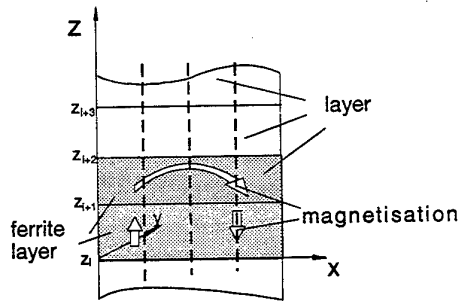
Fig.1 General analysis model with non-homogeneous magnetisation
