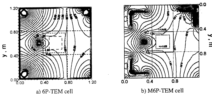
a) 6P-TEM cell b) M6P-TEM cell <Fig.1 Uniformity of the electric field inside the cross section>
