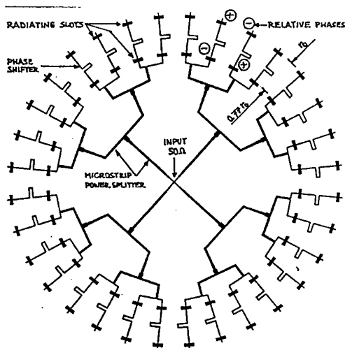
Fig. 1 Layout of the distribution network
