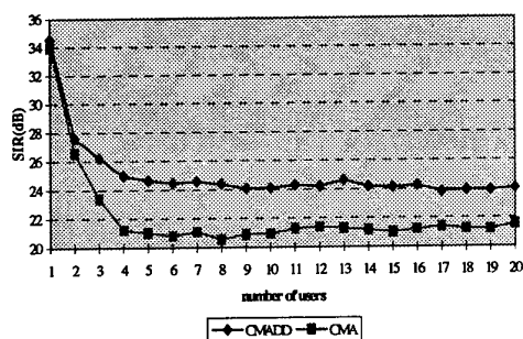
CMA algorithms for DS-CDMA
