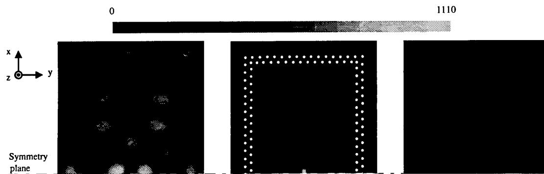
Fig. 1: E_z field in a complete reflective box.
