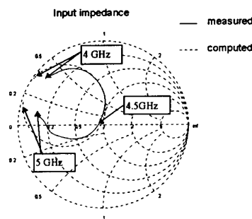
Figure 2 : Input impedance
