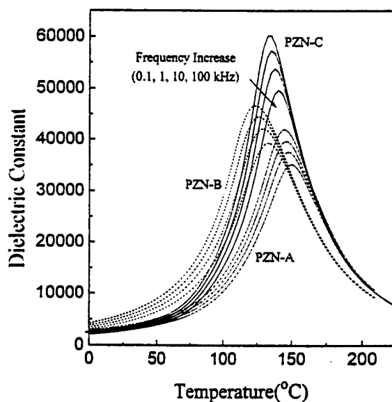
Fig. 4. Temperature dependence of dielectric constant for (111) oriented \text{Pb}(\text{Zn}_{1/3}\text{Nb}_{2/3})\text{O}_3 crystals.
