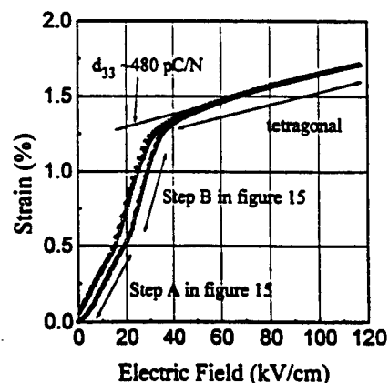
FIG. 17. Strain vs E -field behavior for (001) oriented PZN-8%PT crystal. Maximum field is limited by voltage limit of the apparatus.
