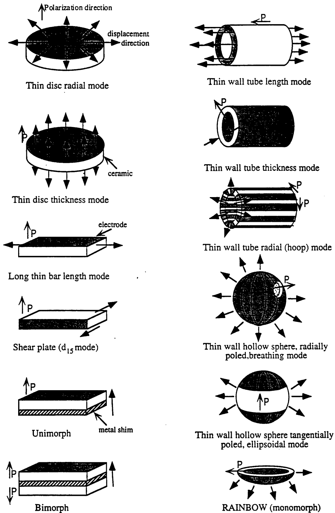
Figure 3. Sensor configurations
