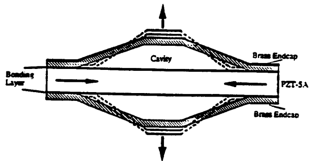
Fig. 1 Schematic of the cymbal transducer.
