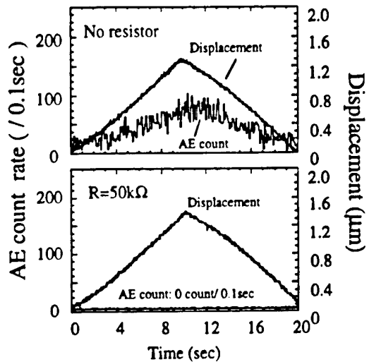
Fig. 4. The AE count and the induced displacement as a function of time with and without R = 50 \text{ k}\Omega .
