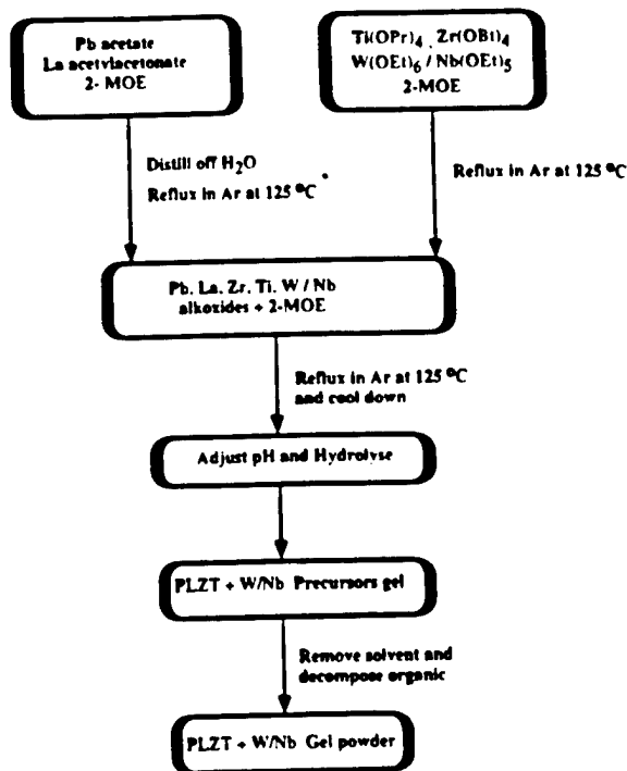
Fig. 2. Flow diagram of sample preparation by sol-gel process. 2-MOE: 2-methoxyethanol, Ti(OPr)_4 : Titanium(IV) isopropoxide, Zr(OBu)_4 : Zirconium(IV) butoxide, W(OEt)_6 : Tungsten(VI) ethoxide, Nb(OEt)_5 : Niobium(V) ethoxide.
