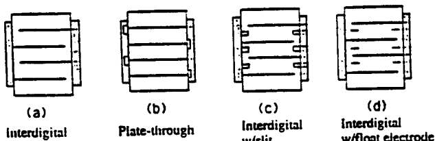
Fig.5. Various electrode configurations for multilayer ceramic actuators.
