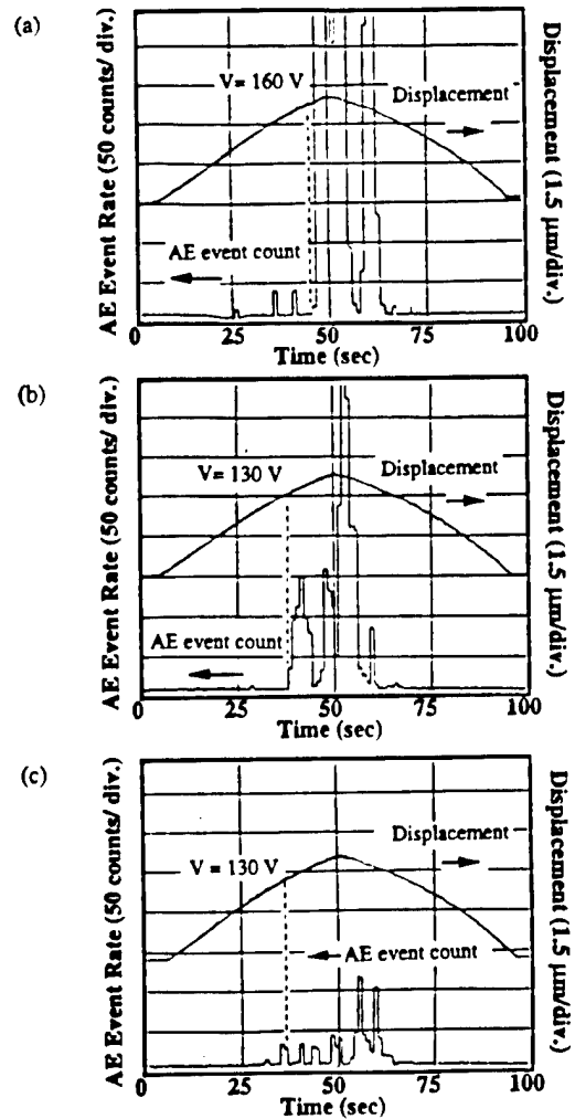
Fig. 8. The AE count and the induced displacement as a function of time: (a) 1st-cycle (b) 2nd-cycle and (c) 10th-cycle.
