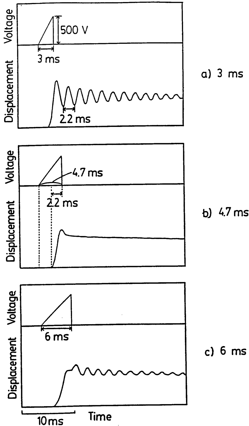
Figure 16. Dynamical response of the tip displacement of the shape memory unimorph with \gamma = 0.063 under various drive pulse conditions [after Furuta, Oh and Uchino (1992)].
