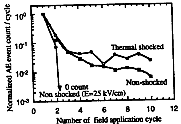
Figure 4. Normalized total AE event count per cycle as a function of the number of field application cycle.
