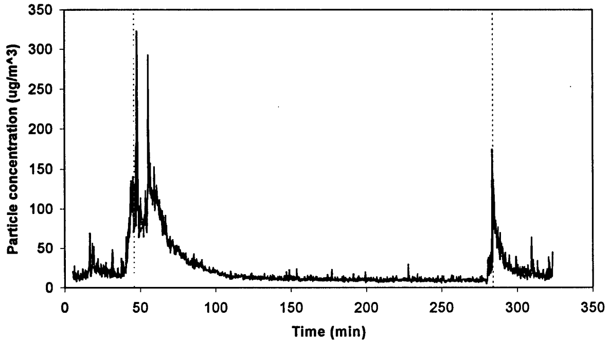
Figure 11. Particle mass concentration profile.
