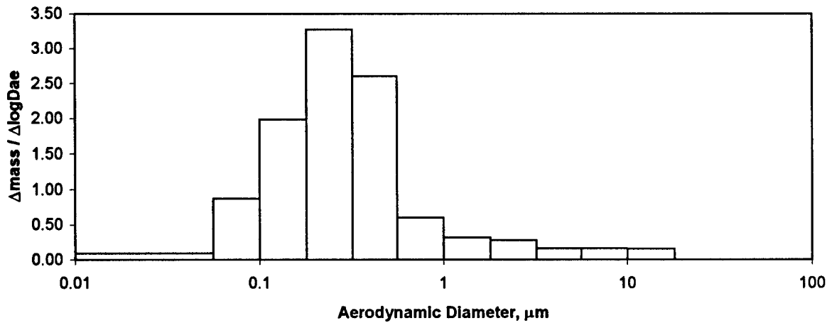
Figure 12. Particle size distribution from the MOUDI impactor.
