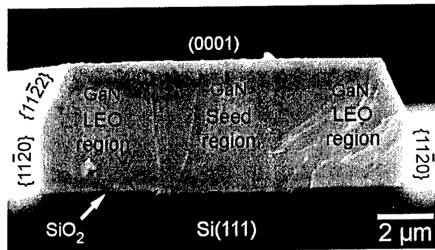
Figure 1 Cross section SEM micrograph of a typical GaN LEO \langle 10\bar{1}0 \rangle -oriented stripe on Si(111) after 60 minutes of growth. Stripes as long as 300 μm were free of cracks, whereas wider stripes resulting from regrowth longer than 120 minutes showed cracking related to thermal expansion mismatch.
