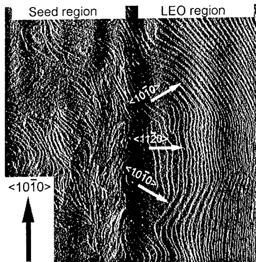
Figure 3 Surface topography of LEO GaN on Si(111) measured by AFM. The contrast in this image is related to the amplitude of the tip vibration during tapping mode imaging. The scan length is 4 μm.
