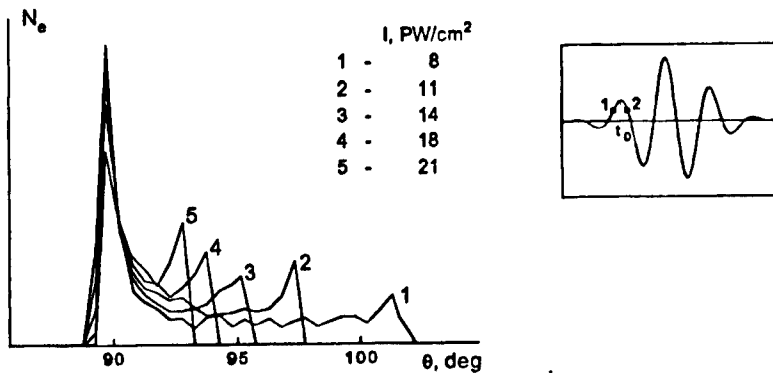
Fig. Electrons \theta -distribution for tunnel ionization of \text{Ar}^{24+} ions by elliptically polarized ( \alpha = 0.04 ) laser radiation with short pulse duration 100 fs, \lambda = 1 \mu\text{m} and different peak intensity I .
