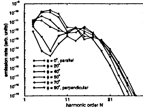
Figure 1: Parameters in a.u.: \omega = 0.076 , I_p = 0.65 , U_p/\hbar\omega = 1.62 , nucl. sep. = 8
