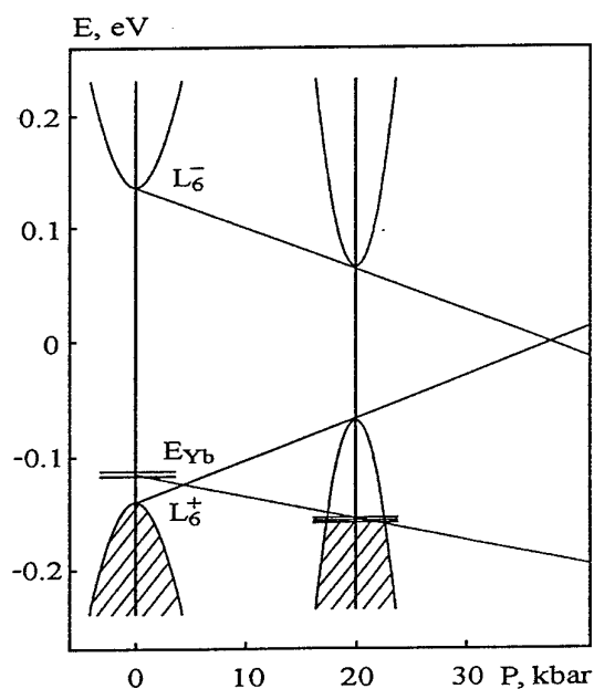
Fig.2. Reconstruction of the energy spectrum of Pb_{1-x}Ge_xTe<Yb> ( x=0.038 ) under pressure at 4.2 K.
