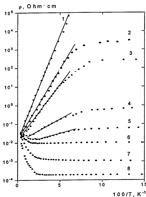
Fig.1. Temperature dependence of resistivity in Pb_{1-x}Ge_xTe<Yb> ( x=0.038 ). P, kbar: 1-0; 2-1.6; 3-2.3; 4-3.2; 5-4.5; 6-6.8; 7-8.7; 8-12.0.
