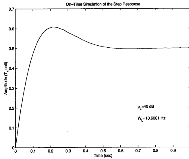
Figure 141 Simulation showing the Step Response of the closed Loop of the BBDLL with, loop Bandwidth W_L = 10.6061 \text{ Hz} , and closed loop signal-to-noise ratio \rho_L = 40 \text{ dB}
