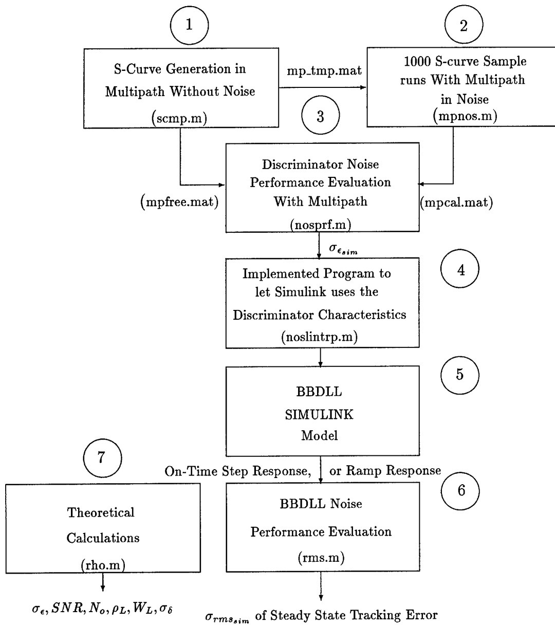
Figure 31 Simulation Block diagram of the standard BBDLL in the the presence of multipath.
