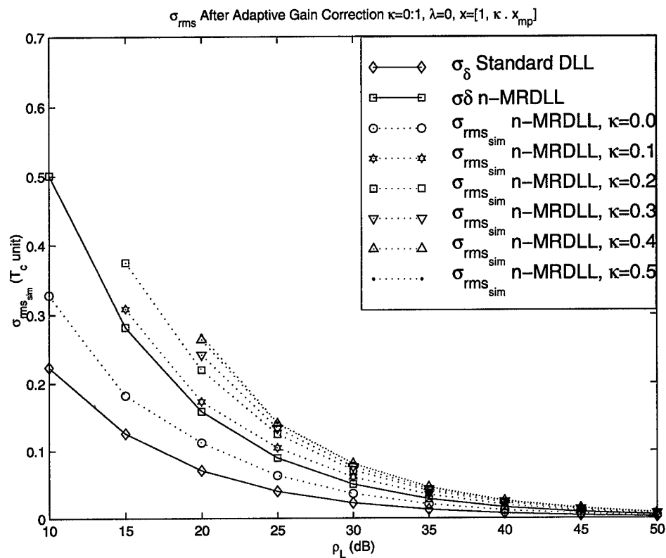
Figure 134 Simulation Results showing the RMS Steady State tracking error \sigma_\epsilon after the adaptive correction, x_{reduction}=[1, \kappa \cdot x_{mp}]
