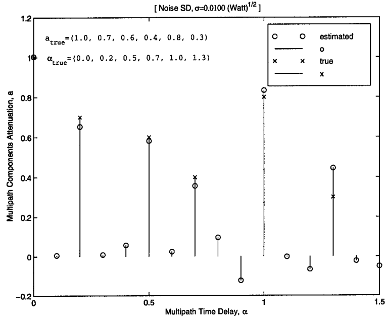
Figure 73 \alpha -Deploying with SD, \sigma=0.0100 \text{ Watt}^{1/2} , Example 5.
