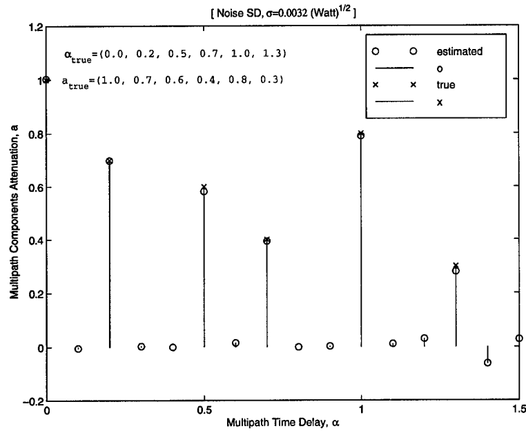
Figure 74 \alpha -Deploying with SD, \sigma=0.0032 \text{ Watt}^{1/2} , Example 5.
