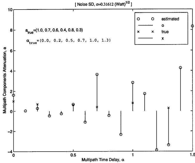
Figure 70 \alpha -Deploying with SD, \sigma = 0.3162 Watt ^{1/2} , Example 5.
