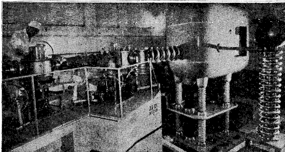
China's first 600,000-volt high energy plasma injector developed by the Hebei Institute of Semiconductors. (Photo by Liu Zhiwei [0491 1807 0251])
