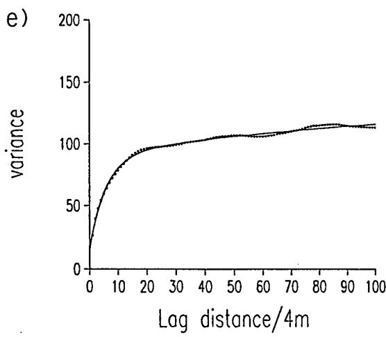
Figure 42: Variograms of channel 4 (Red) from 1 m data for the S part of study area: a) 1 in 2 rows, b) 1 in 2 columns, c) 1 in 2 average, d) 1 in 3 average, e) 1 in 4 average. The symbols are the experimental semivariances, and the lines are the fitted models.
