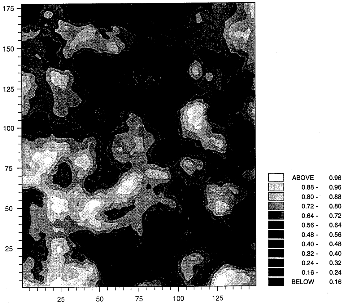
Figure 15: Map of long range kriged estimates after filtering for the A. P. Hill study area: NDVI, SPOT data.
