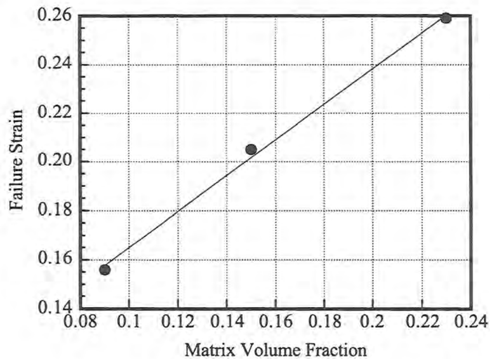
Figure 7. Comparison of Shear Strains to Failure for WHAs With Three Different W Contents (Matrix Volume Fractions).
