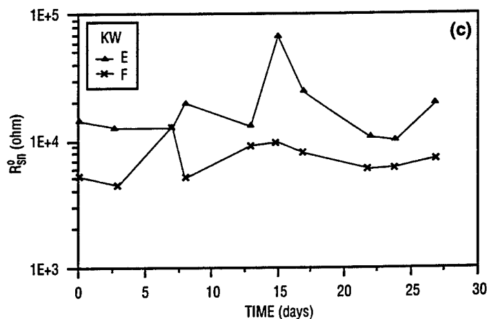
Fig. 21. Time dependence of R_{Sn}^0 for JJ-series samples with artificial defects exposed at KW.
