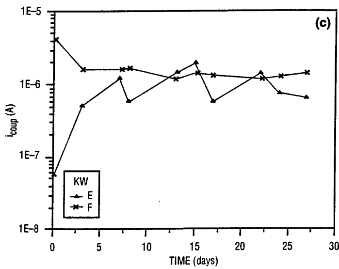
Fig. 20. Time dependence of i_{\text{coup}} for JJ-series samples with artificial defects exposed at KW.
