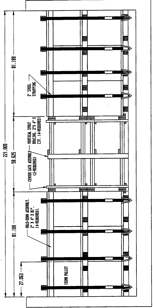
SIDE VIEW
