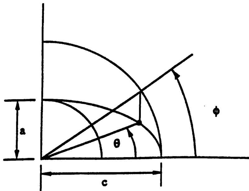
FIGURE 2. DEFINITION OF PARAMETRIC AND PHYSICAL ANGLES
