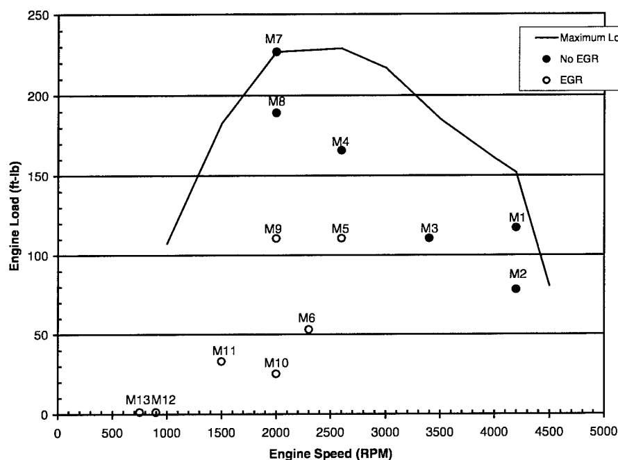
Figure 5. Test Points
