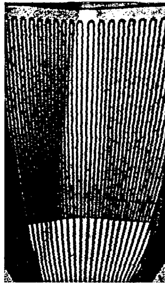
Figure 6.4-2. Rockwell Science Center LBU scan of rocket nozzle
