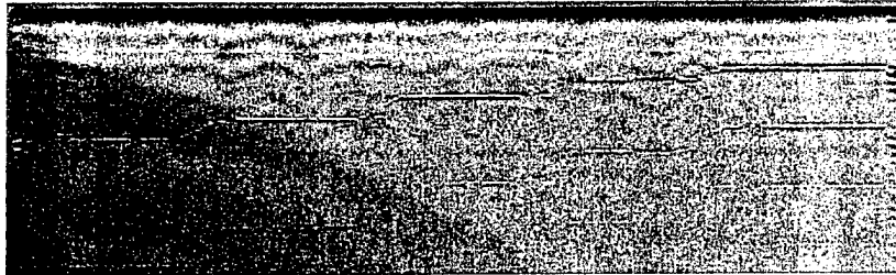
Figure 5.2.7-12. LUIS B-Scan taken from Tool Side
