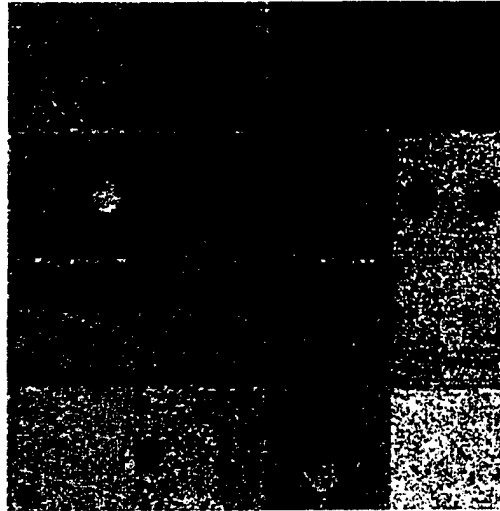
Figure 5.2.15-2. LUIS TOF image of matrix composite standards showing graphite inserts
