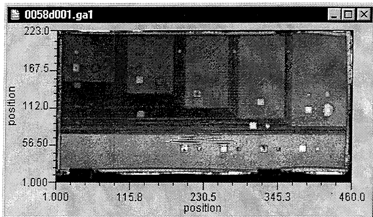
Figure 4.2-1. Example initial amplitude C-scan image
