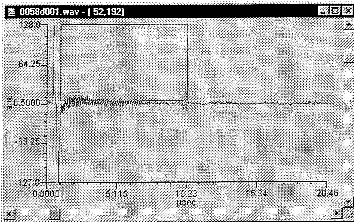
Figure 4.2-5. Waveform at thickest section of part
