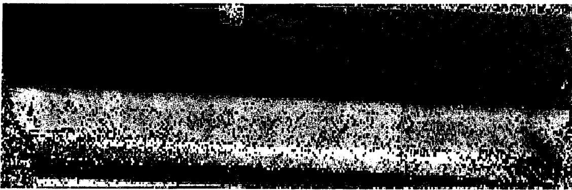
Figure 5.1.8-3. LUIS Time of Flight Image from Curved Leading Edge of Composite Aileron Segment
