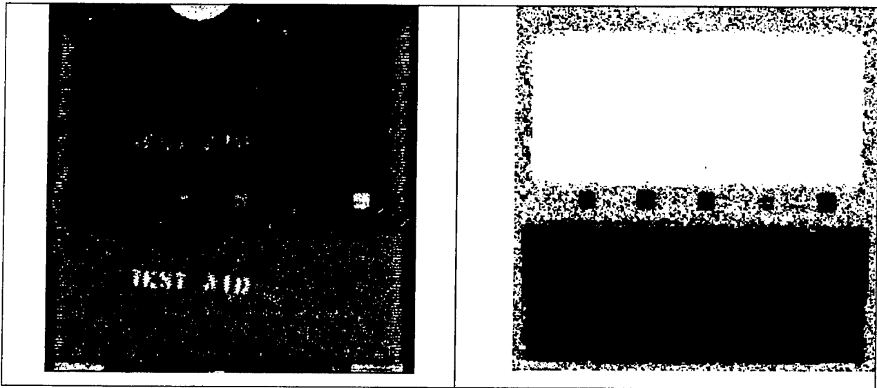
Figure 5.2.1-2. LUIS bag-side amplitude C-scan
