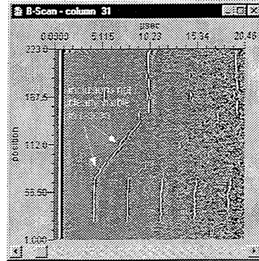
Figure 4.2-28. Vertical B-scan
