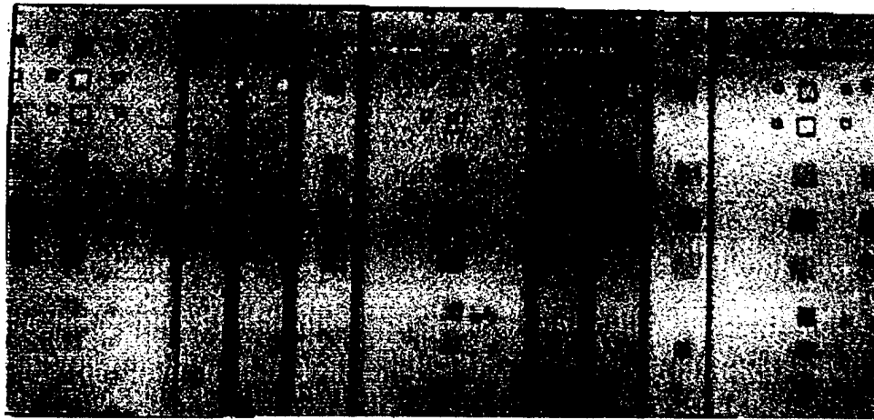
Figure 5.1.2-3. LUIS peak amplitude image of standard 2-A, tool-side scan after painting
