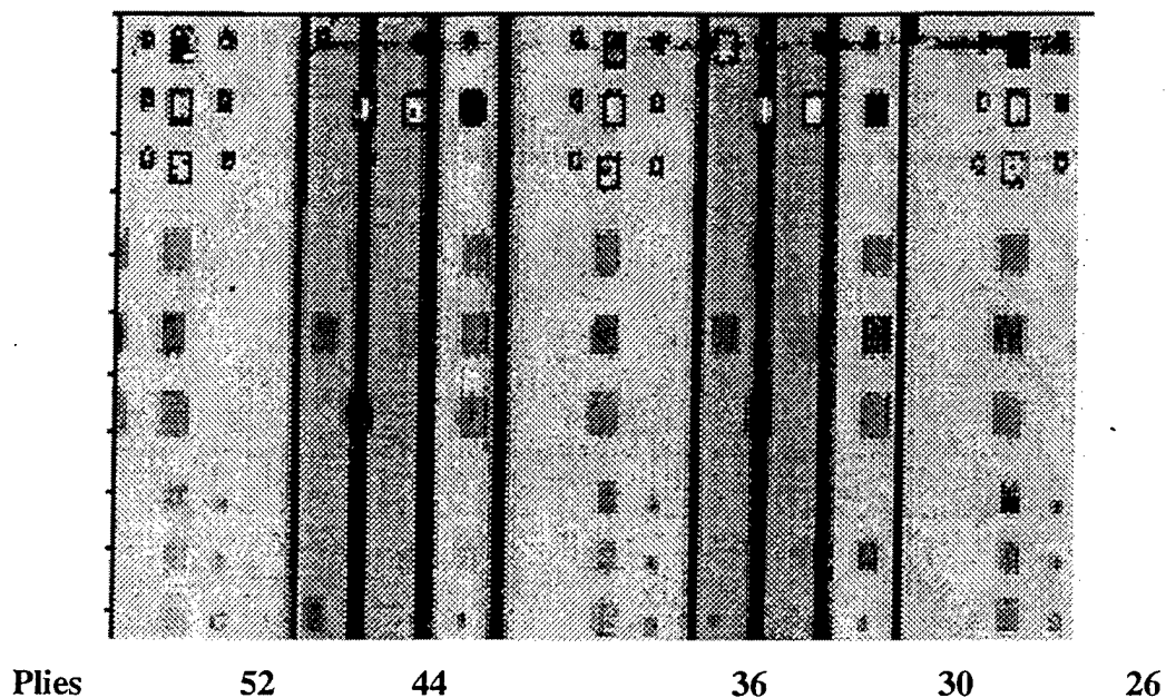
Figure 5.1.2-2. 3.5 MHz Bubbler peak amplitude pulse echo image, 777- 2-A, tool-side scan
