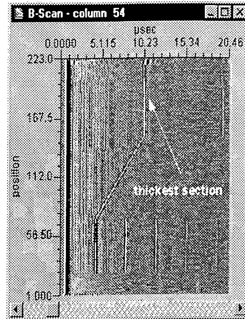
Figure 4.2-4. Example vertical B-scan image
