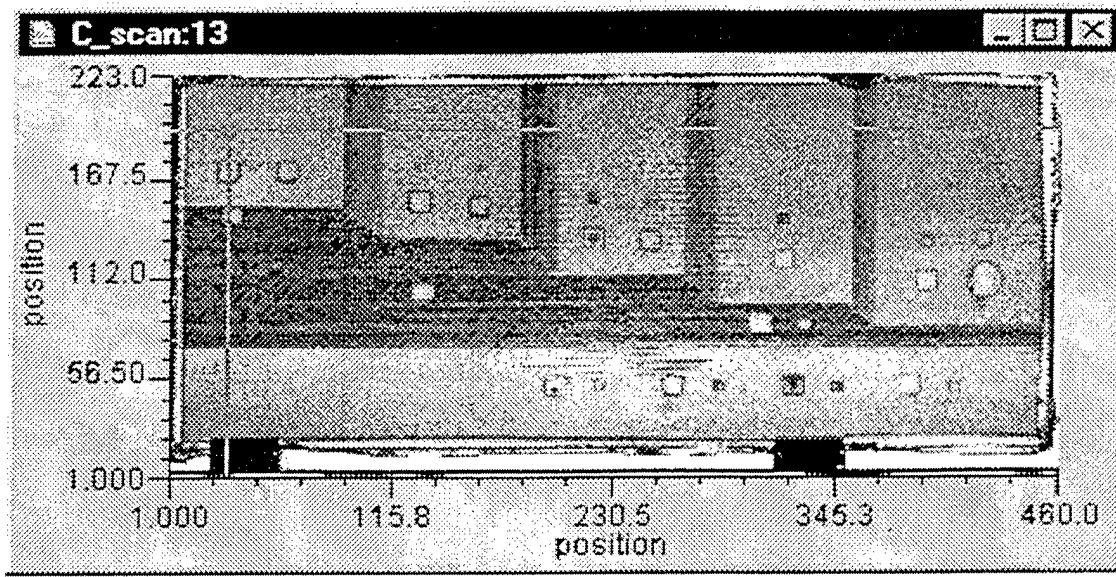
Figure 4.2-26. Position of cross-section for B-scan views
