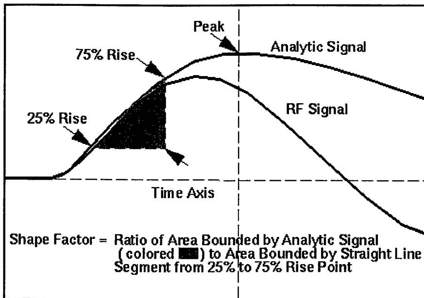
Figure 6.1-2. Shape Definition
