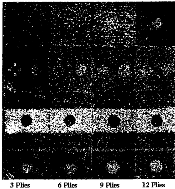
Figure 5.2.15-4. LUIS TOF image of composite standards
