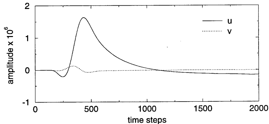
Figure 5: Flow response to ramped actuator motion
