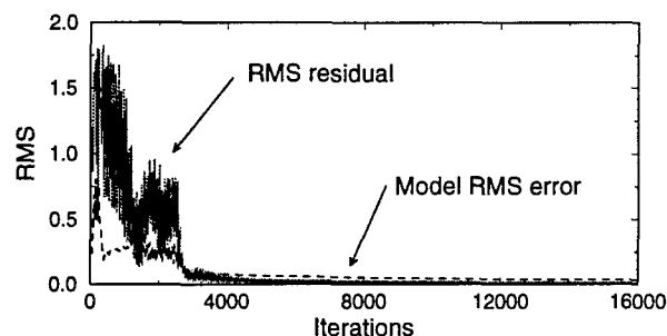
Figure 3: Convergence history of on-the-fly training of inverse model
