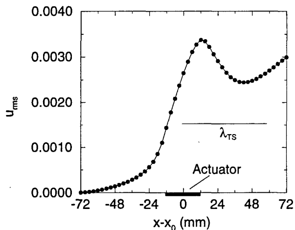
Figure 4: Distribution of u_{rms} along the centerline for sinusoidal actuation at 73 Hz with an amplitude of 0.02 mm. The horizontal line shows the TS wavelength.
