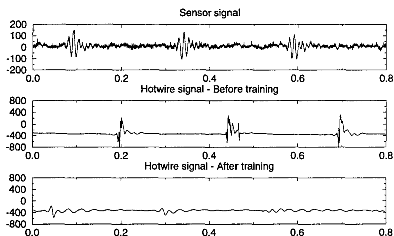
Figure 6: Feedback control of wave packets: before and after training
