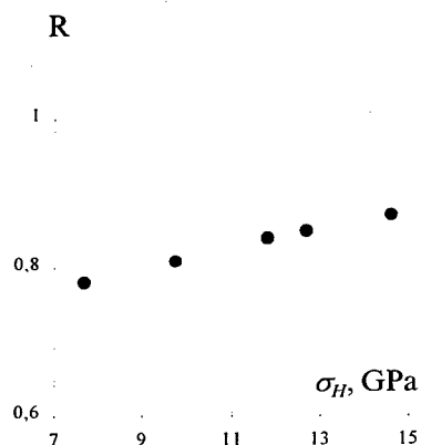
Fig. 4. Parameter R , correlating with damage, vs shock wave amplitude \sigma_H . - calculation, ••• - test
