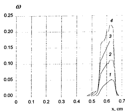
Fig. 3. Distribution of damage \omega along sample thickness at different time moments:
