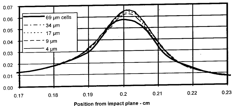
Figure 4 Variation of Damage with Position for various cell sizes Impact in AL 1145 at 185.6 m/s, 0.318 cm target
