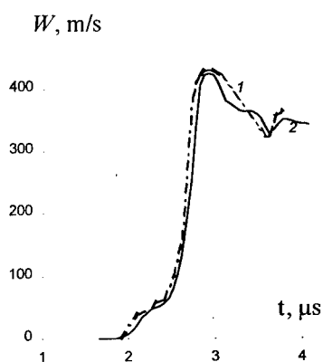
Fig. 1. Sample free surface velocity W vs time.
