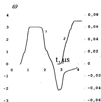
Fig. 2. Stresses \sigma and damage \omega in the fracture zone vs time. 1 - \sigma(t) , 2 - \omega(t)
