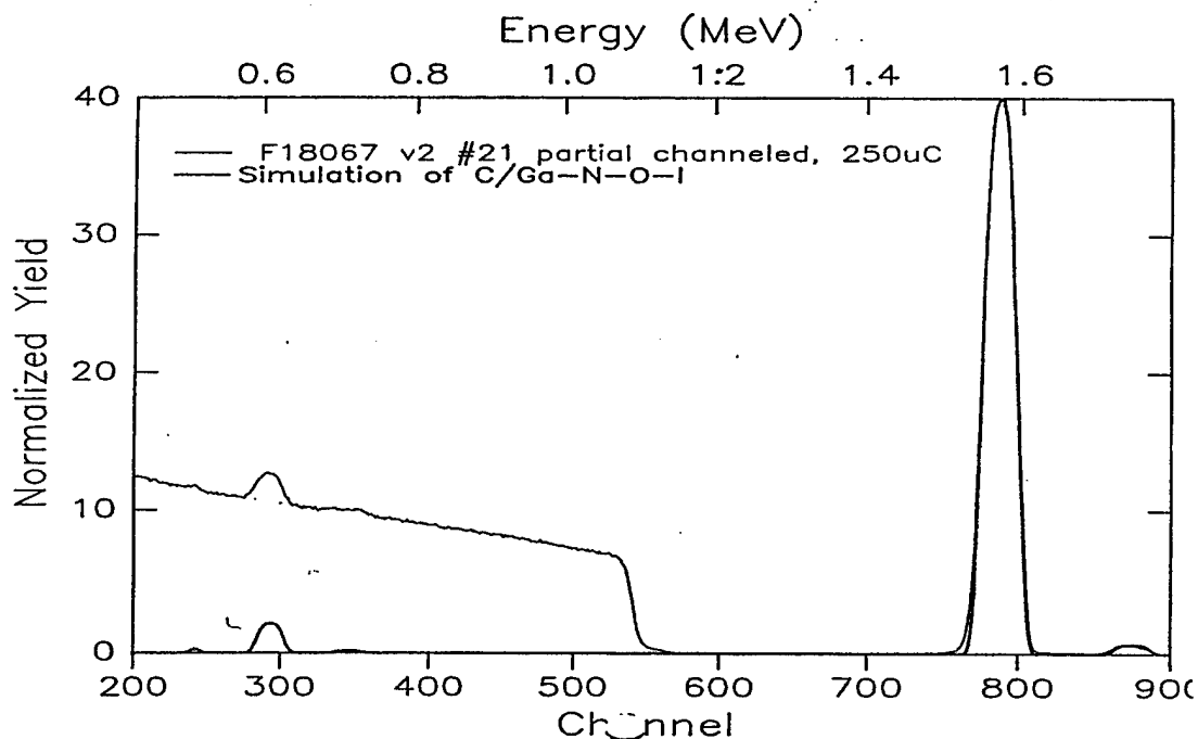
Fig. 4 RBS Results
