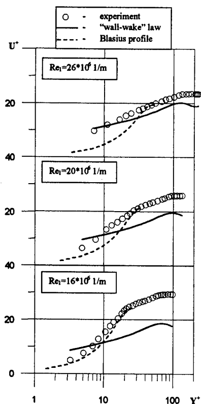
Fig.3 Velocity profiles for X=48\text{mm}
