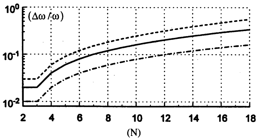
Fig. 2b. The frequency bandwidth (\Delta\omega / \omega) as a function of (N) ; 2 \leq N \leq 18 . [cf. Eq. (13b).] -\cdot-\cdot- \gamma_o = \eta = 0.01 ; — \gamma_o = \eta = 0.02 ; ----- \gamma_o = \eta = 0.03 .
