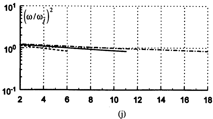
a. \gamma = 0.4 . [cf. Eq. (13a).]
