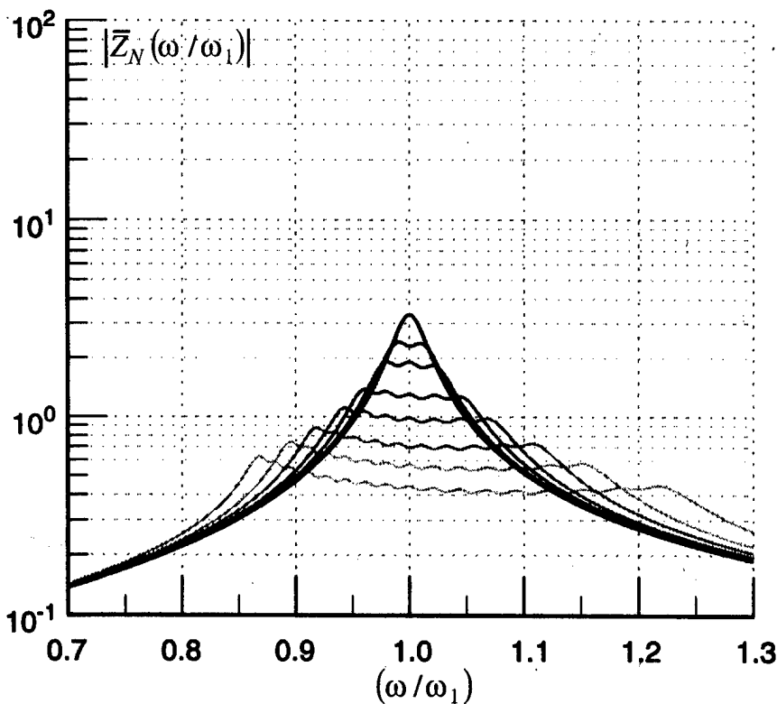
b. \gamma_0 = \eta = 0.02 . [cf. Eq. (13b).]
