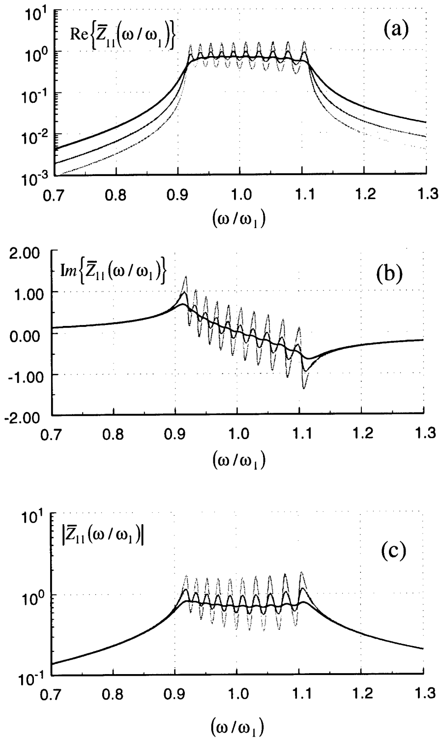
Figs. 7. Normalized joint impedance \bar{Z}_N(\omega/\omega_1) as a function of (\omega/\omega_1) of a set of (N-1) = 10 sprung masses. [cf. Eq. (20).] The set is defined by N = 11 , by a = 10 , by \gamma_o = \eta = 0.02 and by \gamma = 0.4 . [cf. Eq. (13a).] Light curves b = (1/3) , darker curves b = (2/3) and darkest curves b = (3/2) . [cf. Eq. (10).] Employs on the average loss factors. [cf. Eq. (9a).]
