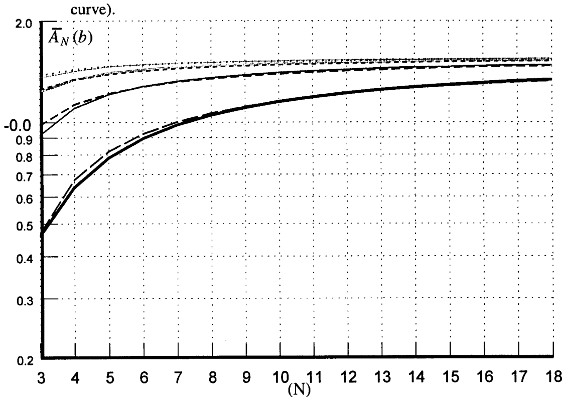
Fig. A2. The undulations-free measure \bar{A}_N(b) as a function of (N) . [cf. Eq (A3).] The values of the overlap factor (b) are: (1/3) (lightest curve), (2/3) , (3/2) and (4) (darkest curve). Superposed is \bar{A}_N(b) as stated in Eqs. (A9) and (A10). These superposed values of \bar{A}_N(b) are depicted by dashed lines.
