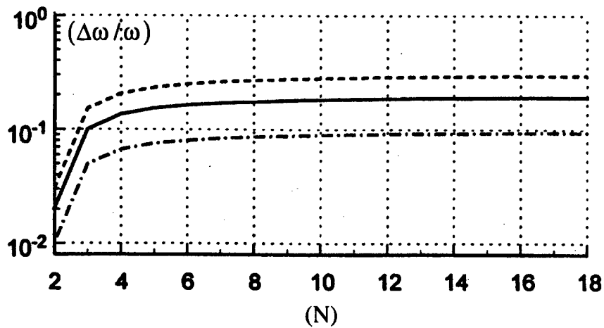
Fig. 2a. The frequency bandwidth (\Delta\omega / \omega) as a function of (N) ; 2 \leq N \leq 18 . [cf. Eq. (13a).] -\cdot-\cdot- \gamma = 0.2, \eta = 0.01 ; — \gamma = 0.4, \eta = 0.02 ; \gamma = 0.6, ----- \eta = 0.03 .
