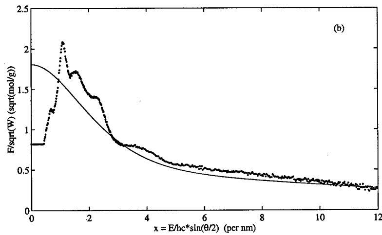
Figure 4: Molecular coherent scattering form factors of (a) pork fat and (b) human breast tissue. The free-gas theory is shown as the solid line and the measured form factors are shown as points. The large differences at lower x values is the reason for having to measure the form factors.
