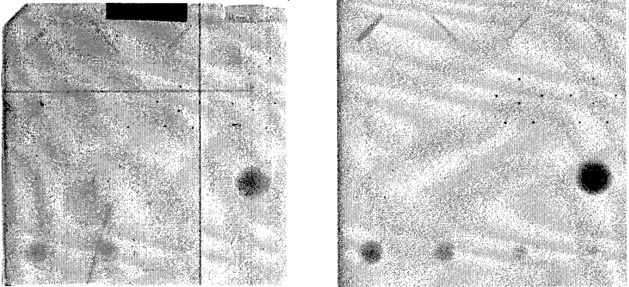
Figure 6: Images of the ACR phantom. Left-image taken with synchrotron radiation. Right-simulation by Monte Carlo. The manufacturer of the ACR phantom acknowledges that there is some variability around the technical standards used in the Monte Carlo.
