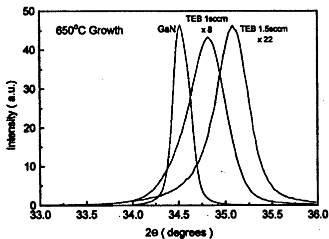
Fig. 2 Changes of position of (0002) reflection of B_xGa_{1-x}N films.
