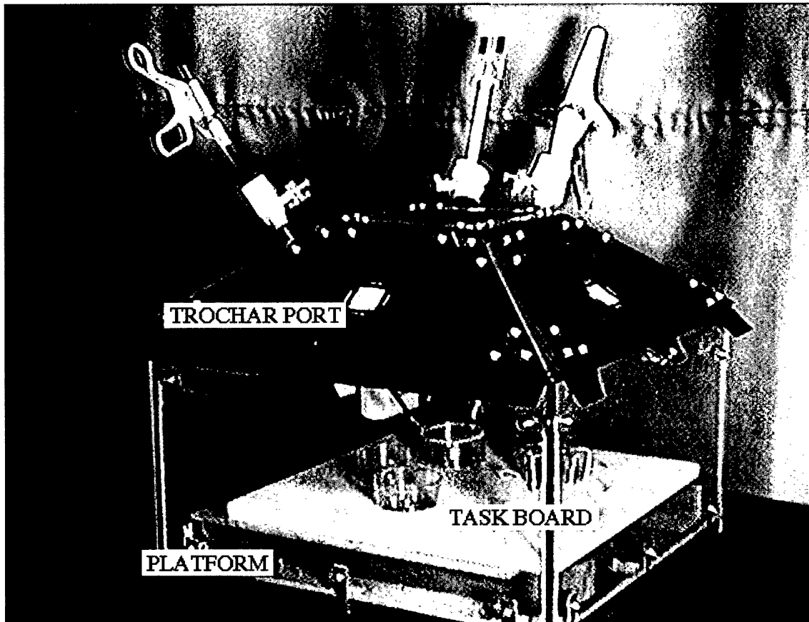
Figure 2.6: Exterior view of simulator
