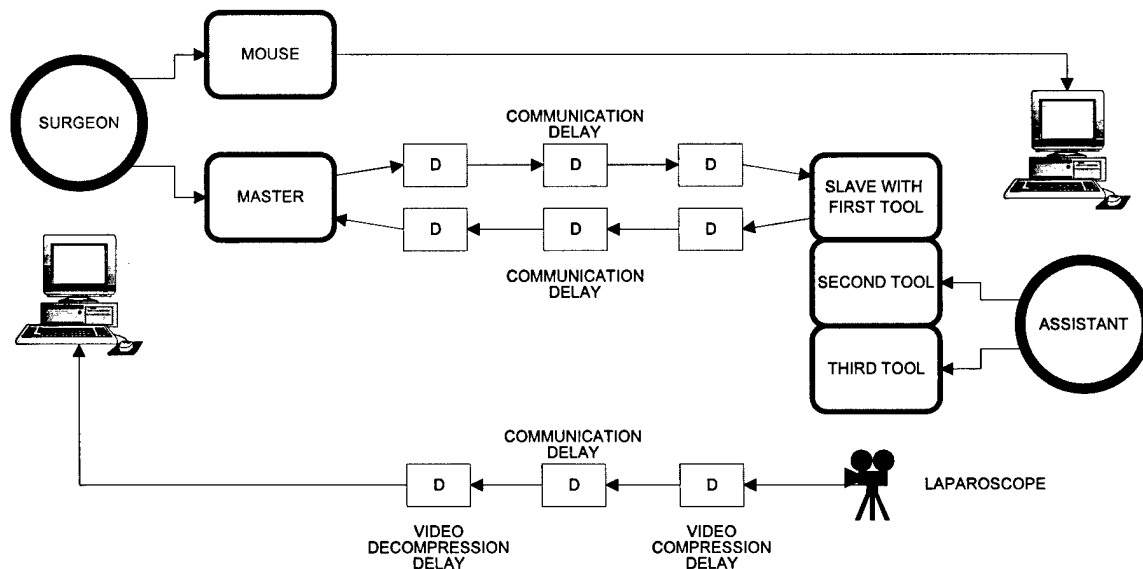
Figure 2.1 Telesurgical System
