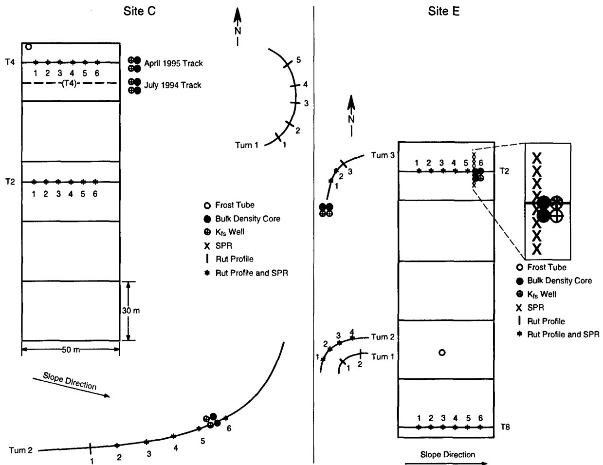
Figure 4. Rut profile transect and soil property measurements locations; the symbol ⊕ indicates the approximate locations of Guelph permeameter wells, ● are soil cores to calculate bulk density (BD), and X indicates permeameter locations (SPR); drawing is not to scale.
