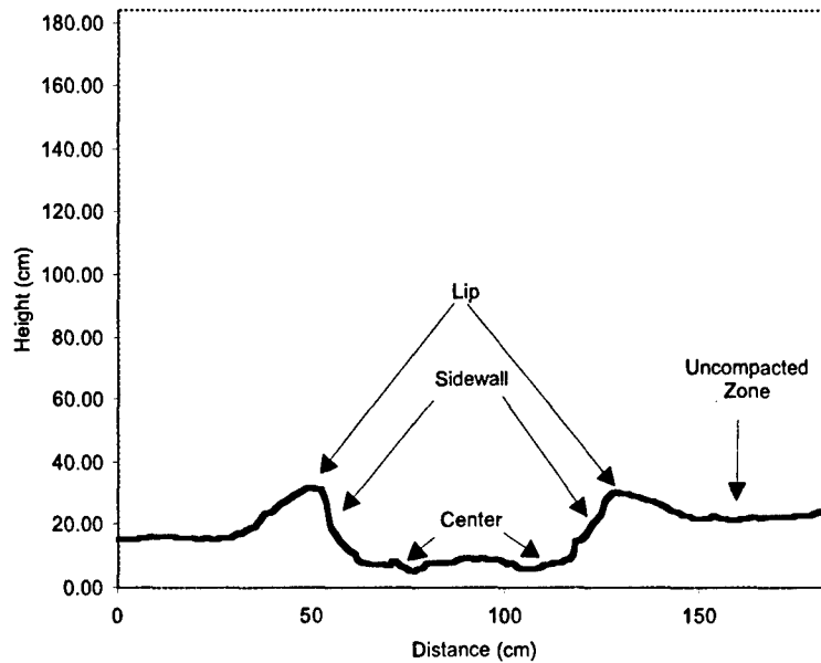
Figure 11. General cross-sectional shape of an M1 Abrams tank rut.
