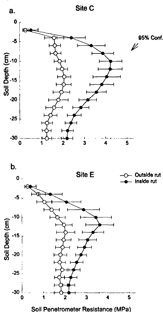
Figure 12. Average soil penetrometer resistances \pm 95\% confidence intervals for profile locations ( n = 17 [site C], 18 [site E]).
