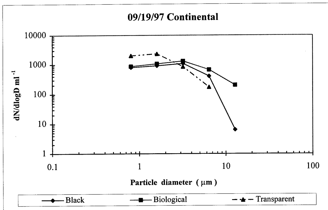
Figure 8. Black, biological and transparent particle size distribution. dN/d\log D per ml vs. diameter ( \mu m ).
