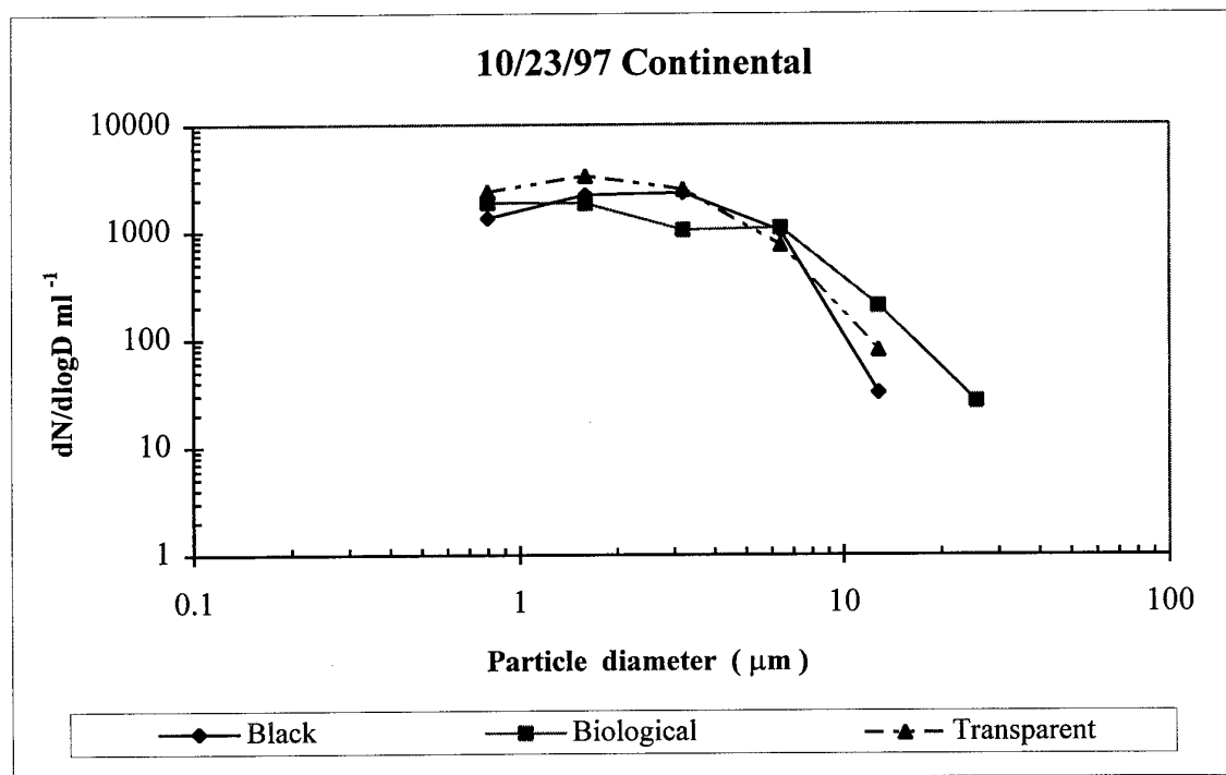
Figure 14. Black, biological and transparent particle size distribution. dN/d\log D per ml vs. diameter ( \mu m ).
