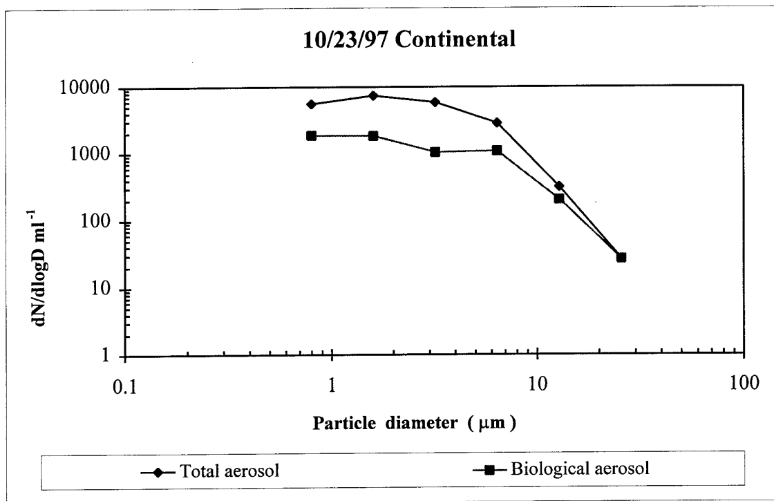
Figure 13. Total and biological aerosol size distribution. dN/d\log D per ml vs. diameter ( \mu m ).
