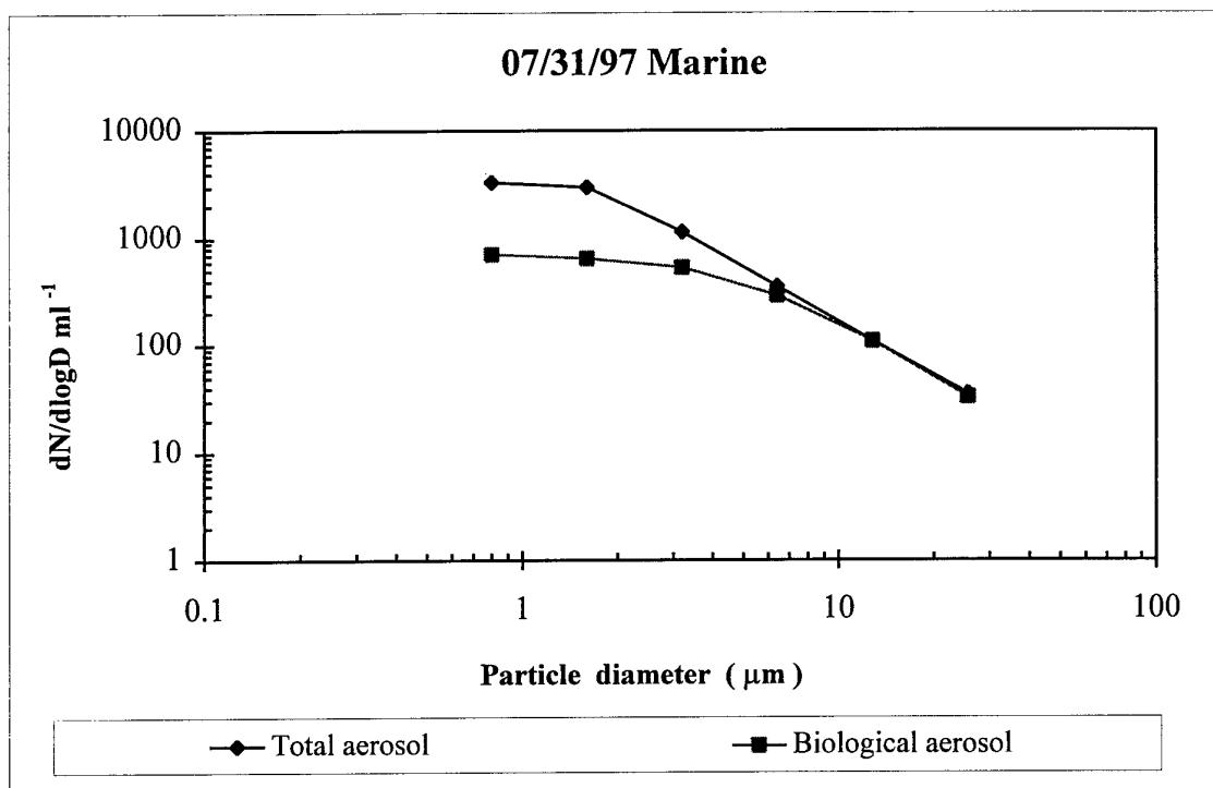
Figure 1. Total and biological aerosol size distribution. \text{dN/dlogD} per ml vs. diameter ( \mu\text{m} ).
