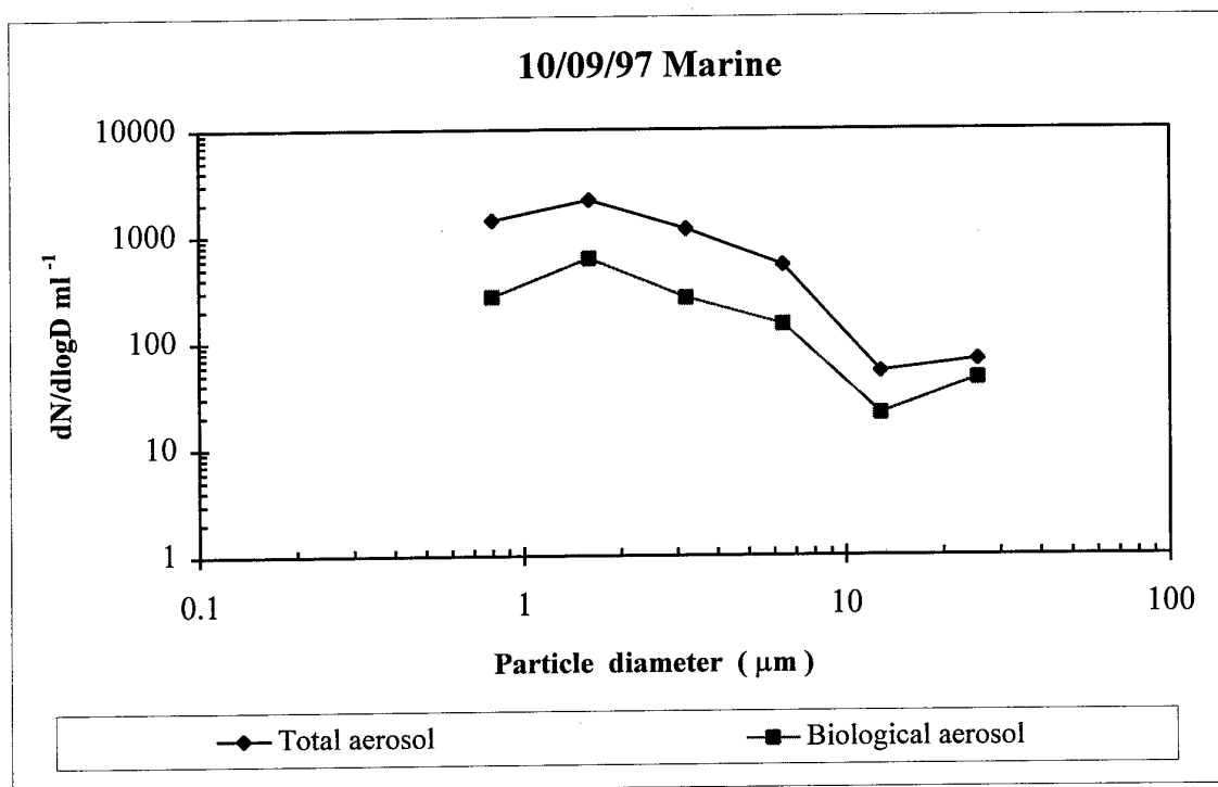
Figure 11. Total and biological aerosol size distribution. dN/d\log D per ml vs. diameter ( \mu m ).
