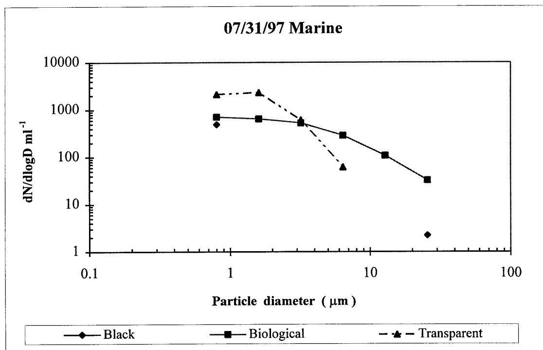
Figure 2. Black, biological and transparent particle size distribution. \text{dN/dlogD} per ml vs. diameter ( \mu\text{m} ).
