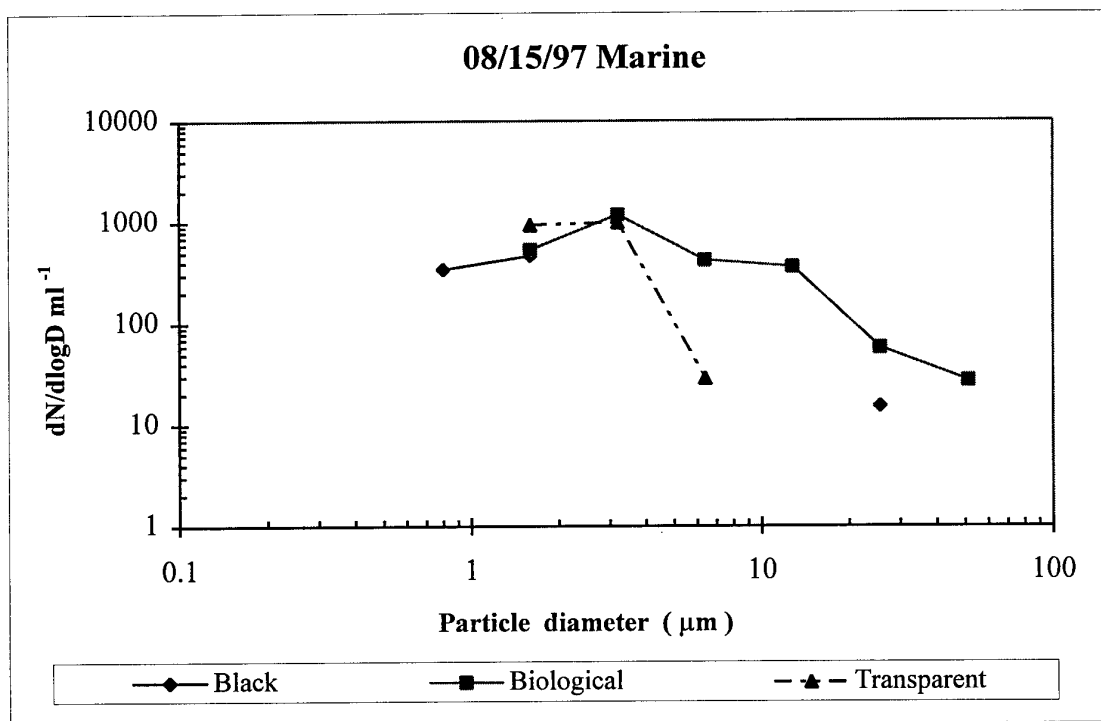
Figure 4. Black, biological and transparent particle size distribution. dN/d\log D per ml vs. diameter ( \mu\text{m} ).
