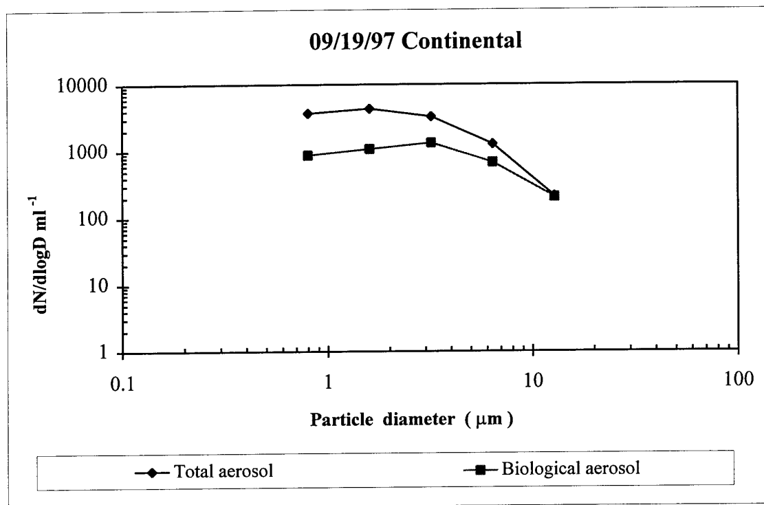
Figure 7. Total and biological aerosol size distribution. dN/d\log D per ml vs. diameter ( \mu m ).
