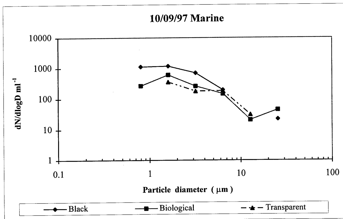
Figure 12. Black, biological and transparent particle size distribution. dN/d\log D per ml vs. diameter ( \mu m ).
