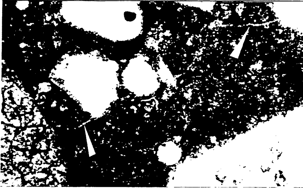
Figure J5. CPAR: Core Sample No. S35-25132, C-3. Thin section photomicrograph detailing microcracks (arrows) in the hydrated cement paste. Plane polarized light, 190 × Mag
