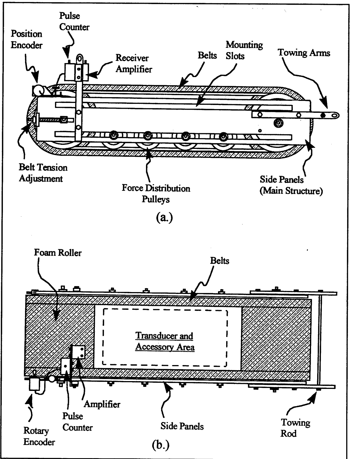
Figure 6. Diagram showing frame of rolling pond and accessories(a) side view (b) top view
