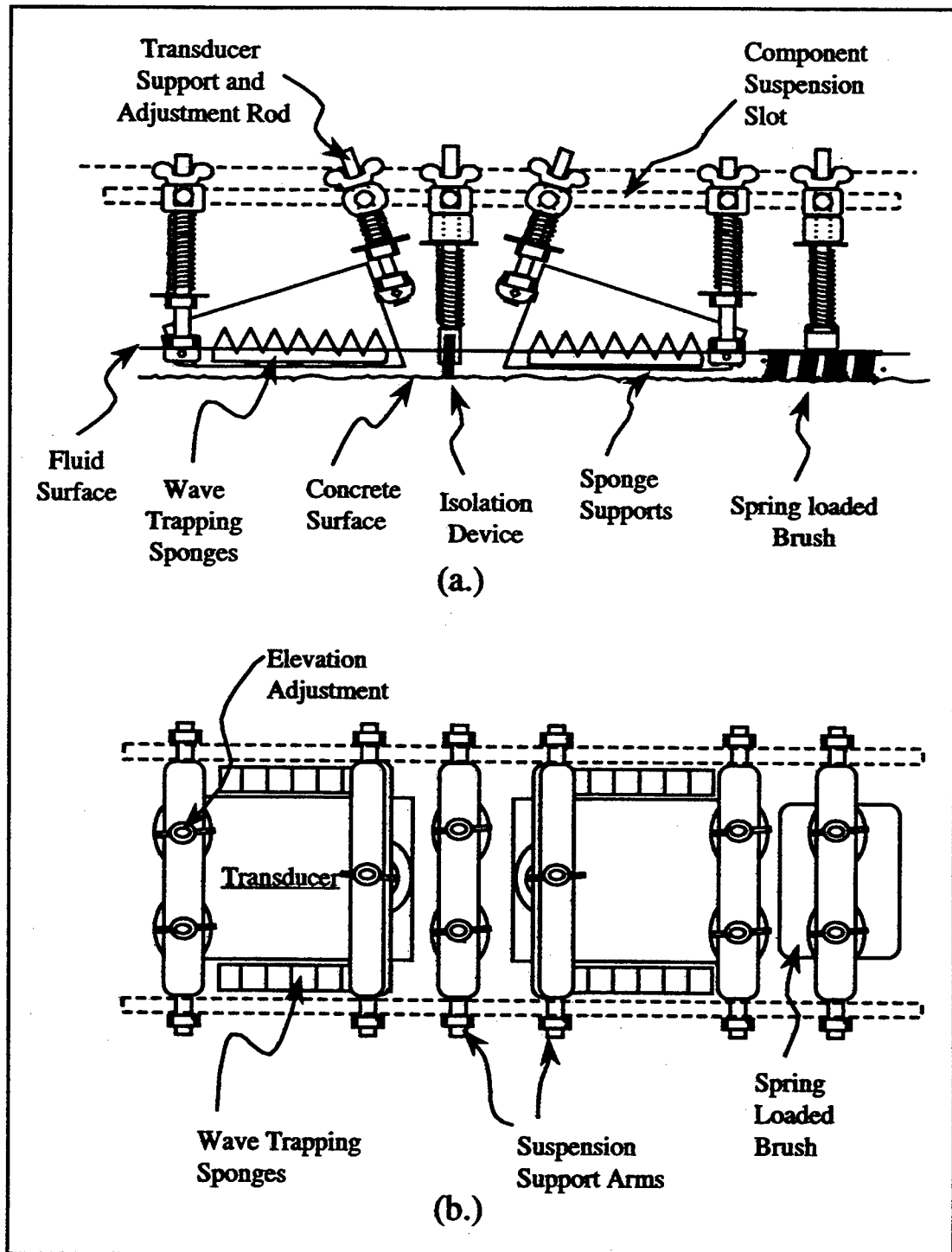
Figure 9. Rolling pond's interior components (a) side view (b) top view
