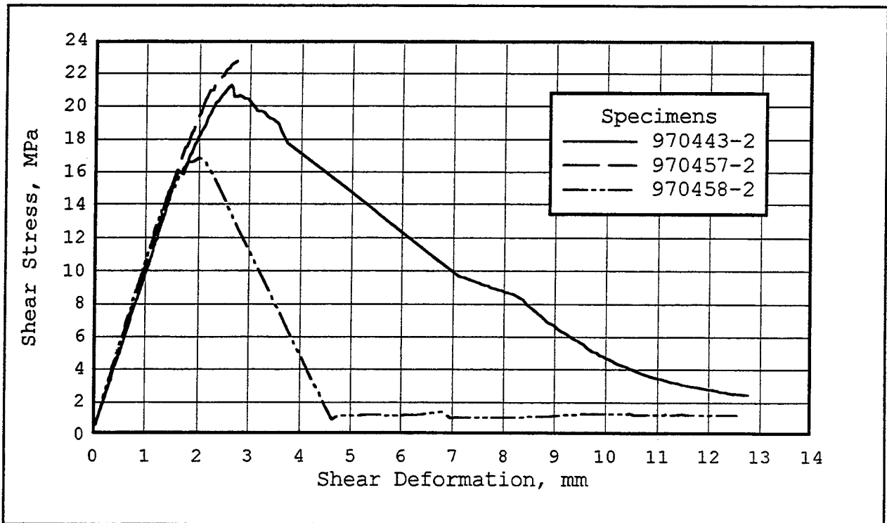
Figure 10. Shear-strength test results for dry mixture at normal stress of 0.8 MPa
