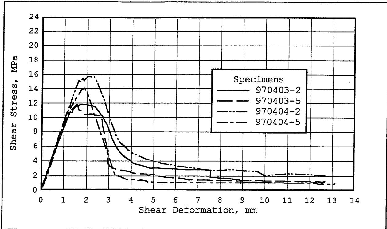
Figure 9. Shear-strength test results for wet mixture at normal stress of 0.8 MPa
