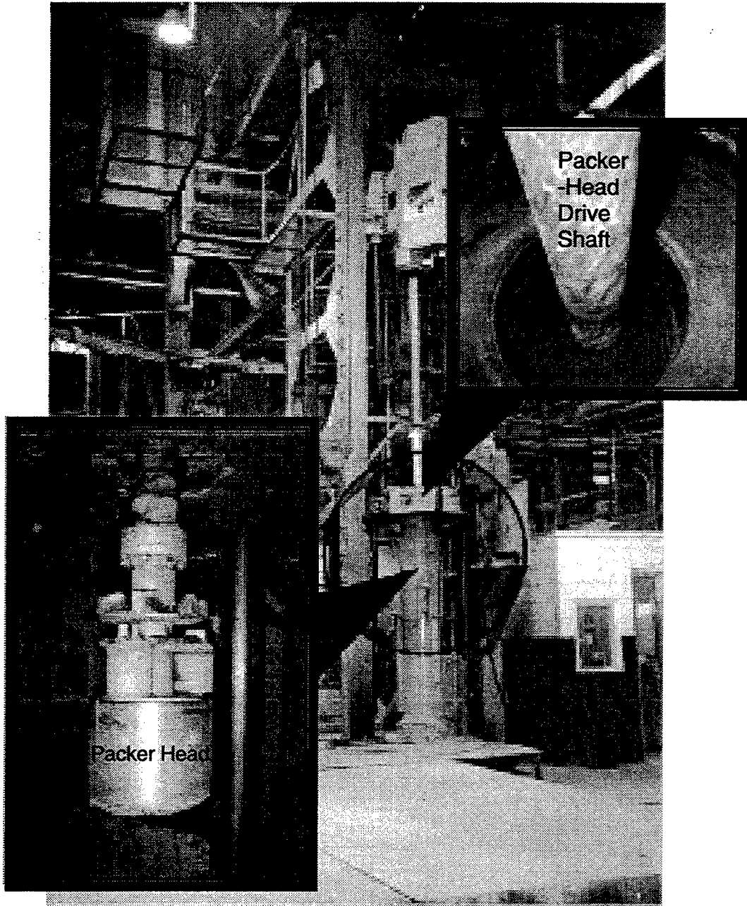
Photo 1. Packer-head equipment
