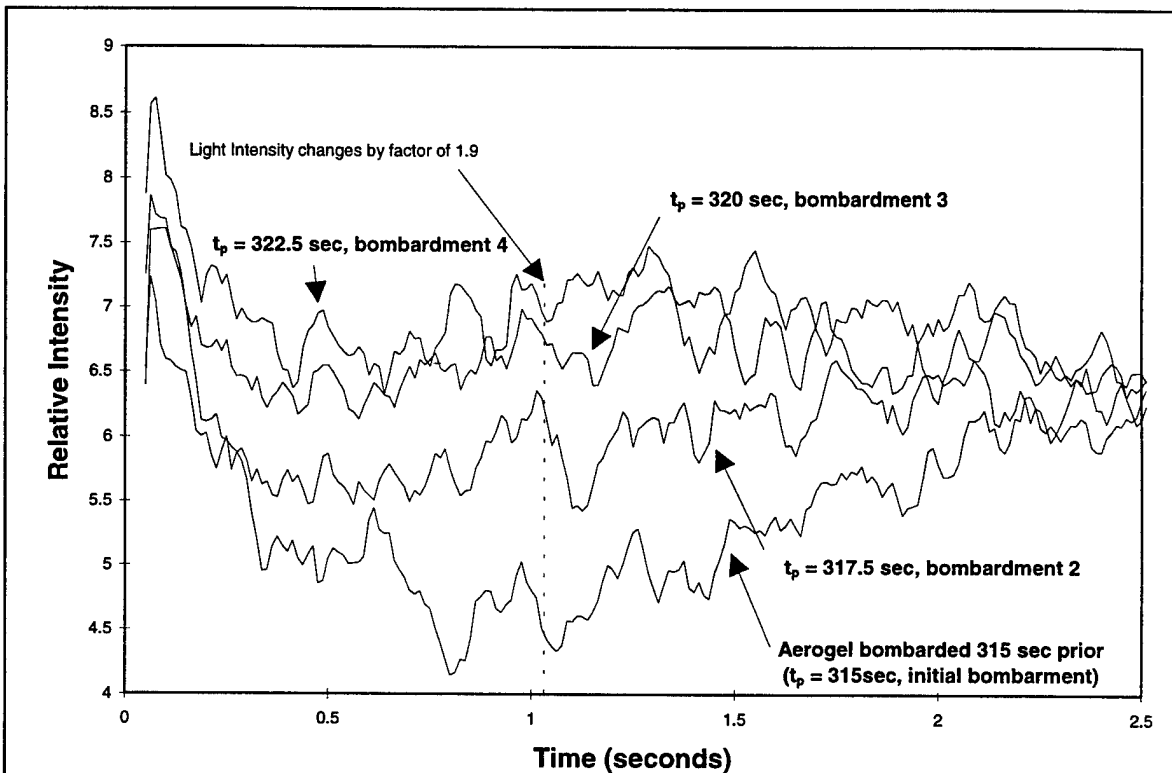
FIGURE 19: FOUR INDIVIDUAL BOMBARDMENTS OF A SHORT TERM TIME DEPENDENT SEQUENCE
