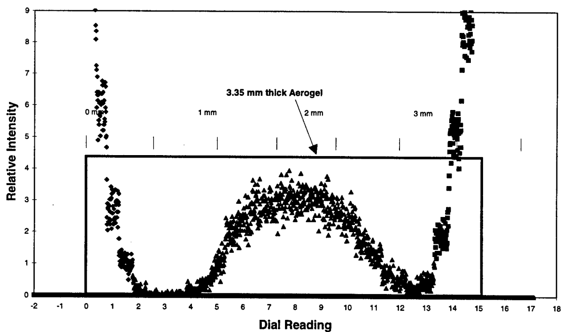
FIGURE 10: LIGHT INTENSITY AS A FUNCTION OF DIAL READING FOR A 'BACK-LIT' AEROGEL
