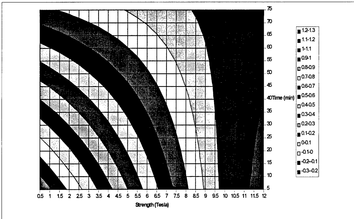
Figure 4-11. Surface and contour plots of the predicted orientation parameter response variable as a function of the field strength and time in the field for a constant B-staging time of 90 minutes.
