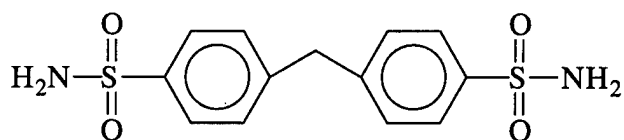
4,4'-methylenebis(benzenedisulfonamide) (MB-BDSA)
