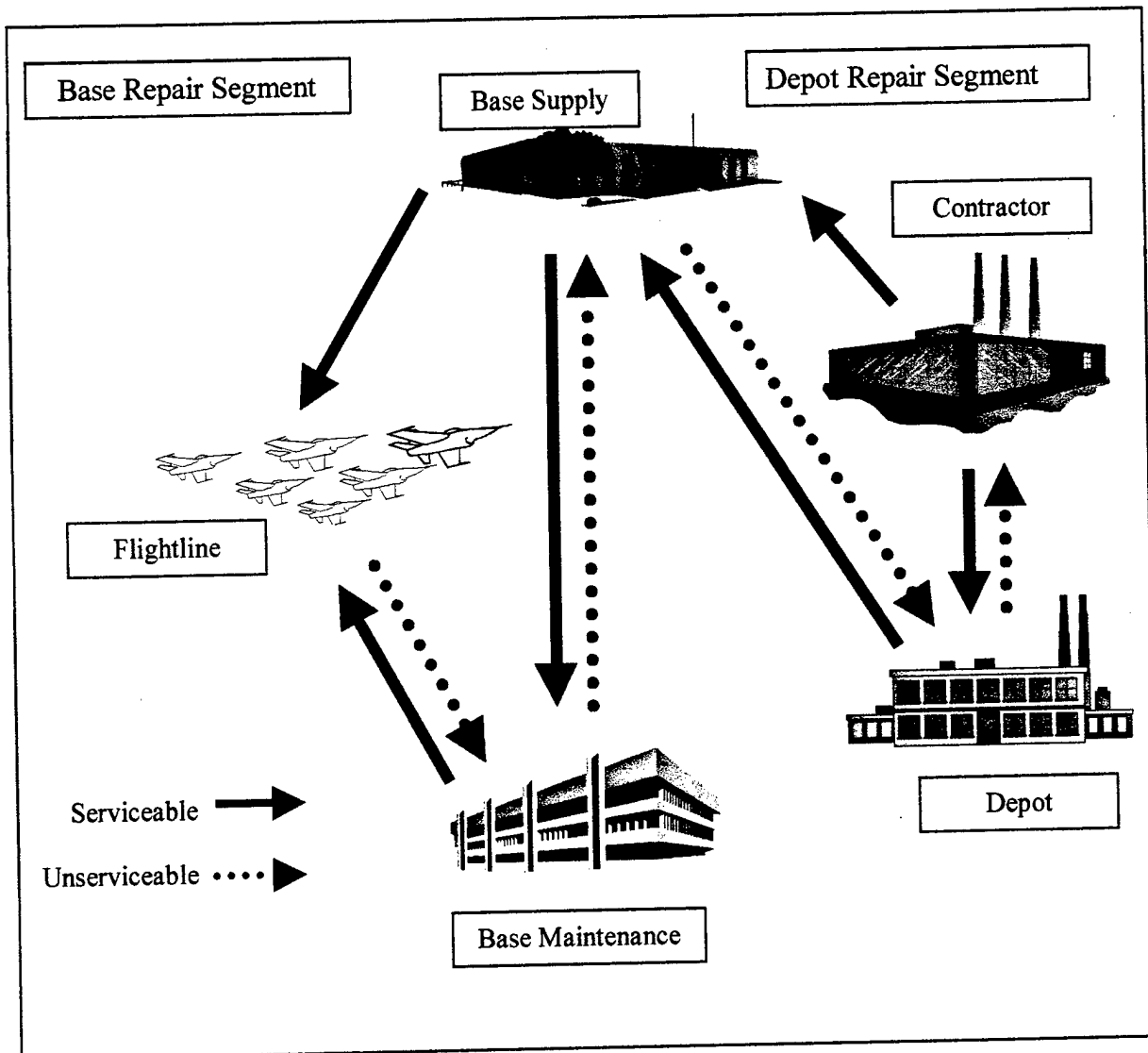
Figure 4-1 Engine Pipeline
