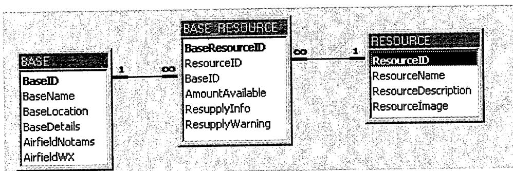
Figure 24. Resource table relationships
