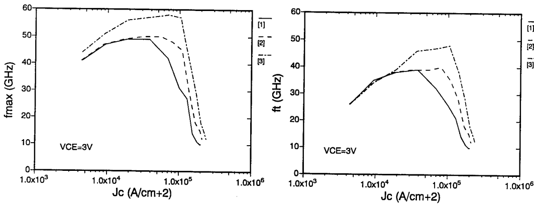
Fig. 3: f_{max} and f_t versus collector current density ([1]: basic structure, [2]: improved thermal surface conductivity between emitter and base contact, [3]: emitter area 2 \times 45 \mu\text{m}^2 )
