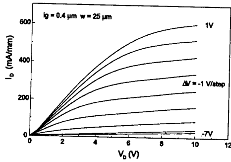
Fig. 2. DC I-V output characteristics at R.T..
