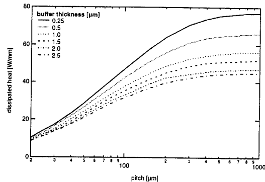
Fig. 5: maximum dissipated power for a max. surface temperature of 200°C
