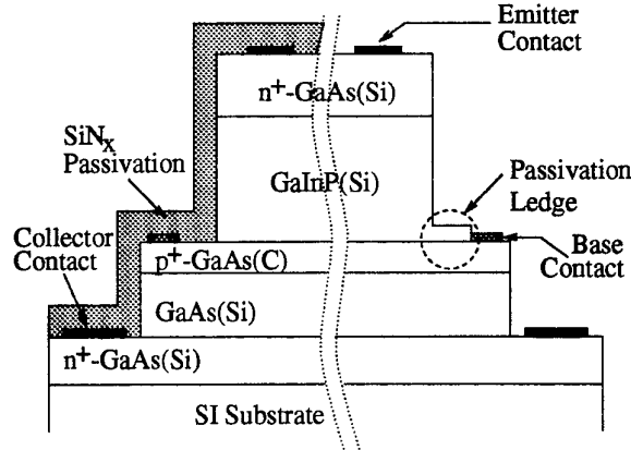
Figure 1: Epitaxial structure of the investigated HBTs.
