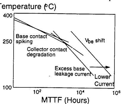
Fig. 6. MTTT as a function of temperature, bias current in an HBT.
