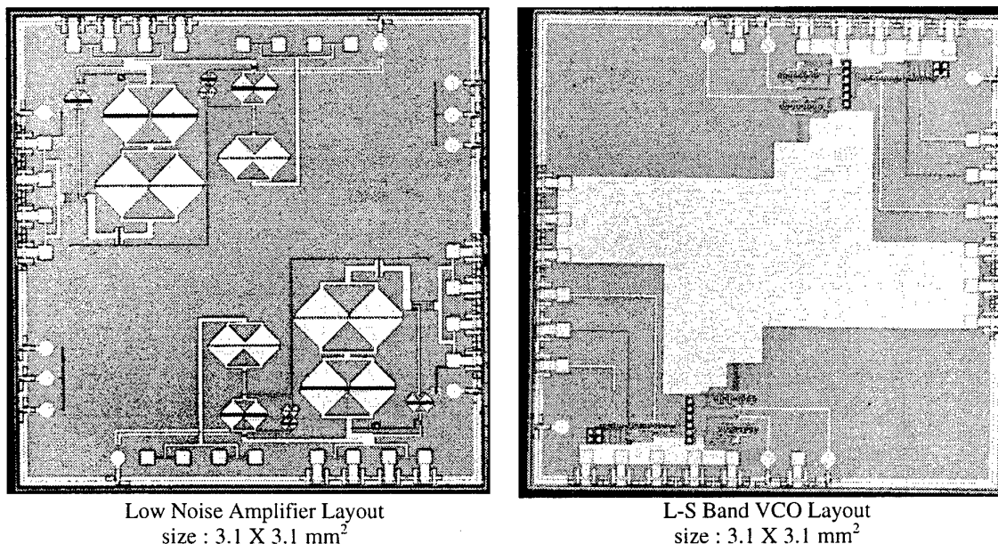
Figure 8 : SiGe MMICs
