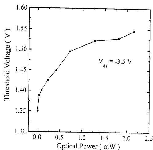
Fig. 3 Threshold voltage vs. optical power
