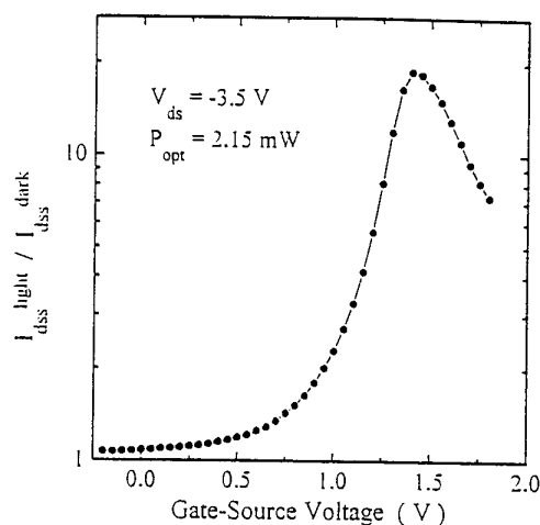
Fig. 4 Ratio of saturated drain currents vs. V_{gs}
