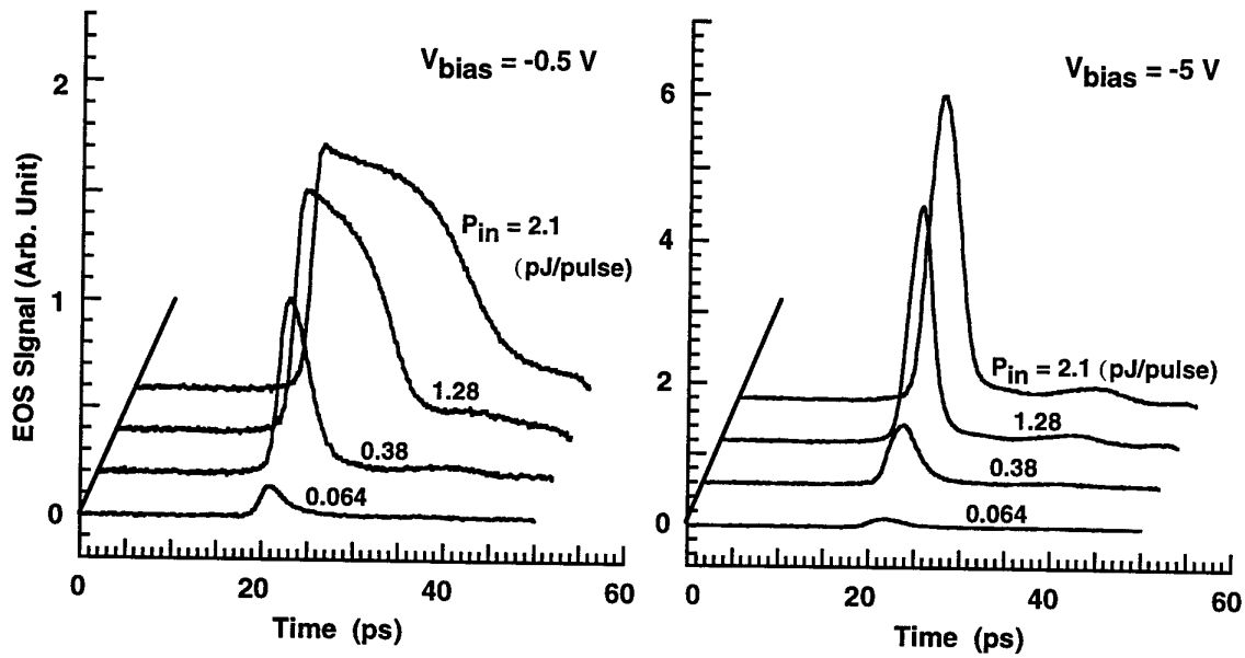
Fig. 2 Photoresponse waveforms of a UTC-PD with optical input level as a parameter (Incident pulse: \lambda = 1.55 \mu\text{m} , FWHM = 790 fs).
