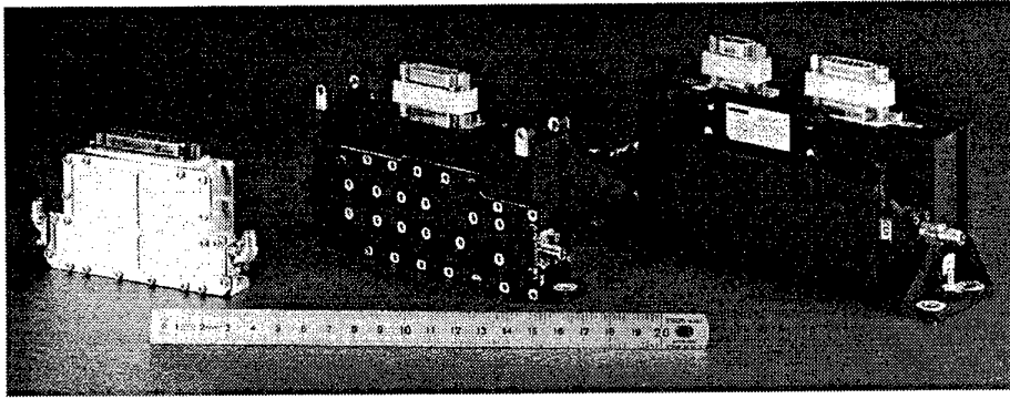
Figure 3: Three generations of CAMP: « Hybrid » with 550g, « MMIC » with 210g and « MCM » with 95g. This represents about 10 years of evolution.
