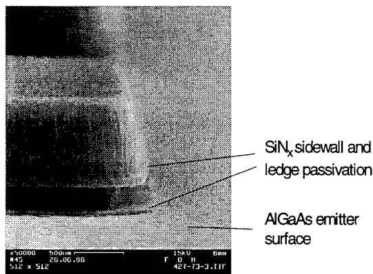
Fig. 1 SEM image of emitter mesa and ledge structure realization
