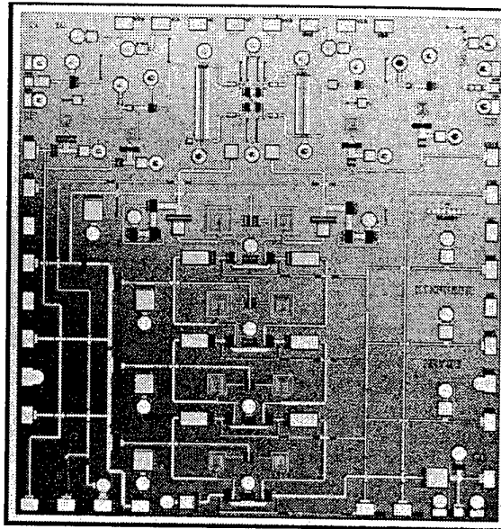
Figure 6 : Ku band microstrip multifunction schematic and layout (size: 4 x 4.1mm 2 )
