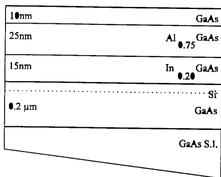
Fig. 1 : Cross-section of HIGFET epitaxy
