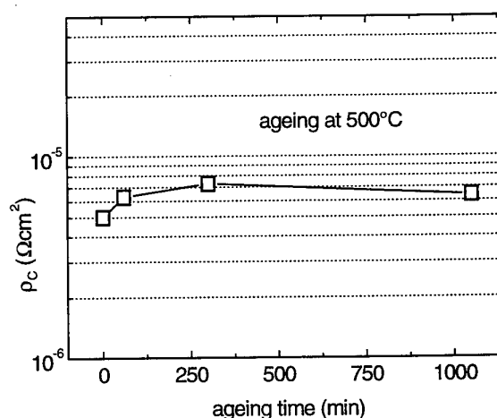
FIG. 2: Specific contact resistance of Ti/WSiN on GaN versus ageing time in \text{N}_2 .
