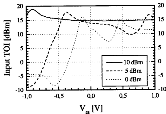
Fig. 2: Measured input third order intercept point of single ended resistive FET mixer vs. bias for different LO power levels.
