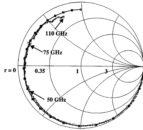
Fig.3 S_{11} versus frequency at zero bias measured (+) and calculated (-).
