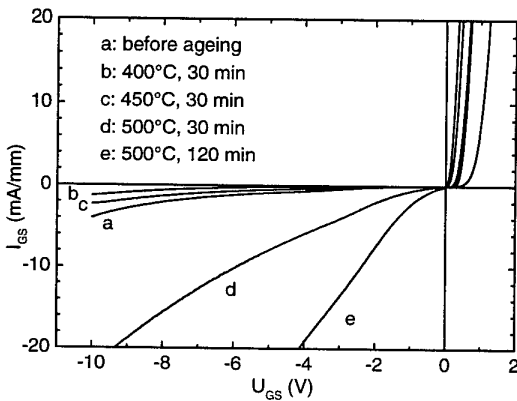
Fig. 3: Gate diode I/V characteristics of a GaN-MESFET before and after ageing.
