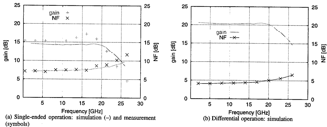
Figure 3: Gain and noise figure of the differential amplifier
