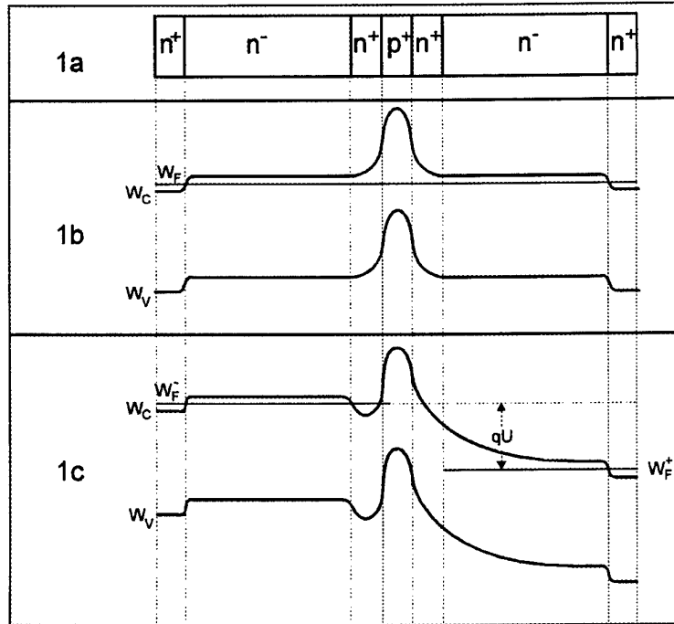
Fig. 1: Schematic representation of a DBV 1a) layers sequence, 1b) energy band structure for zero bias, 1c) energy band structure for applied bias voltage
