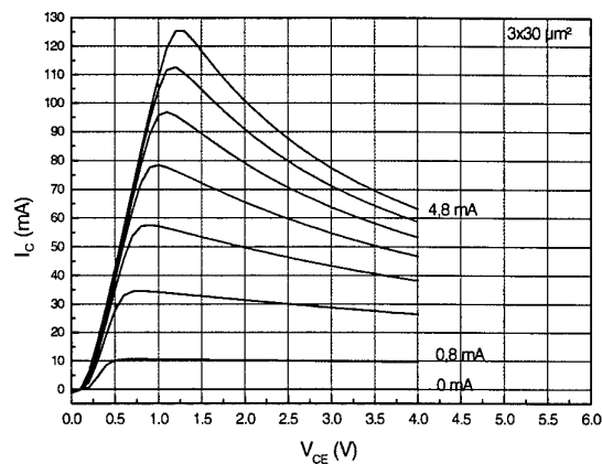
Fig. 2 Common emitter I-V characteristics of a 3 \times 30 \mu\text{m}^2 HBT
