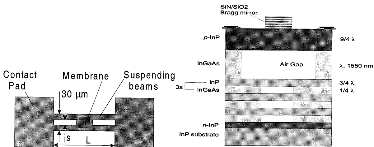
Figure 1: Schematic of a micromechanically tunable Fabry-Pérot filter, left: top view, right: cross section.
