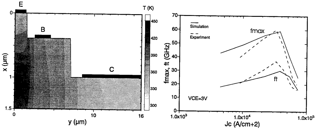
Fig. 2: Temperature distribution at V_{CE} = 3 \text{ V} and J_C = 2 \cdot 10^5 \text{ A/cm}^2
