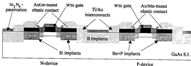
Fig. 2 : Complementary HIGFET technology
