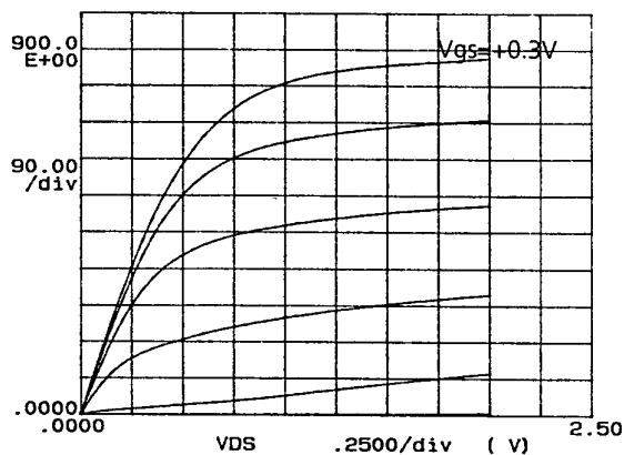
Fig. 3: I-V characteristics of passivated 0.15 \mu\text{m} passivated InP-based-HEMT, with gate bias steps of -0.3 V.
