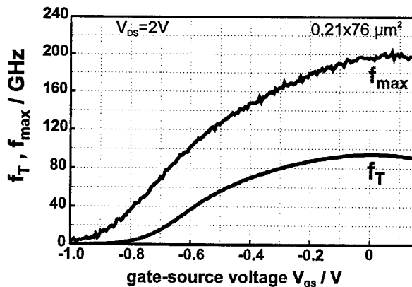
Fig.1: High-frequency behaviour ( f_T and f_{\max} (MAG)) of e-beam gate HEMT versus V_{GS} , measured at 25 GHz (gate length: 0.21 \mu\text{m} , gate width: 76 \mu\text{m} ).
