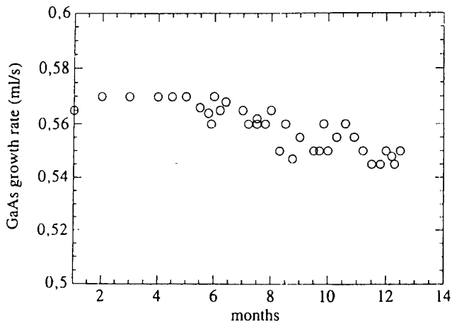
Fig. 1 Growth reproducibility demonstrated by the evolution of growth rate during a period of 12 months at a fixed temperature and TEG pressure set point A
