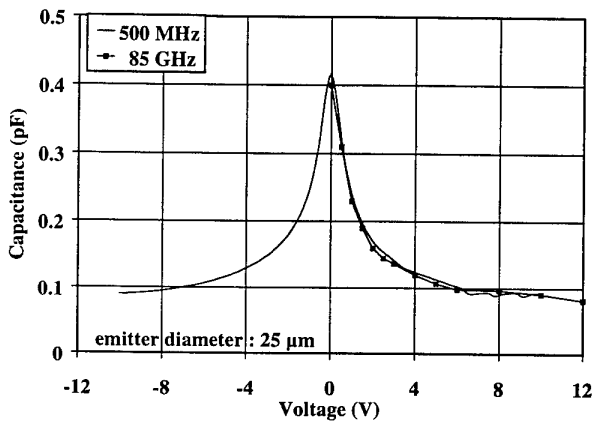
Fig2: C-V curve measured @ 0.5 and 85 GHz
