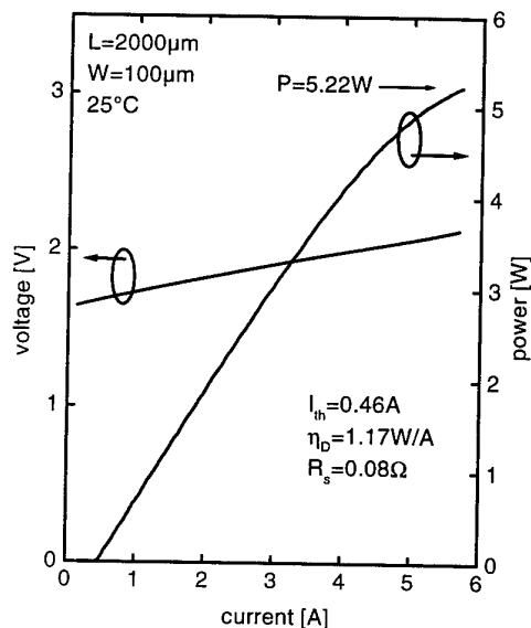
Fig. 3: CW power current voltage characteristic of a 100\text{ }\mu\text{m} \times 2000\text{ }\mu\text{m} single laserdiode
