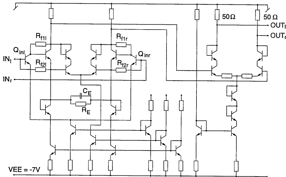
Figure 2: Schematic of the differential amplifier
