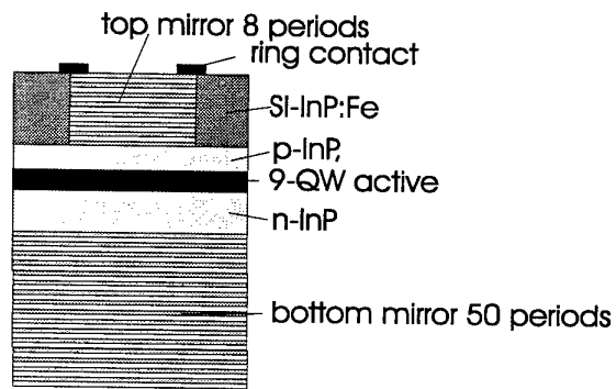
Figure 1: RCLED structure
