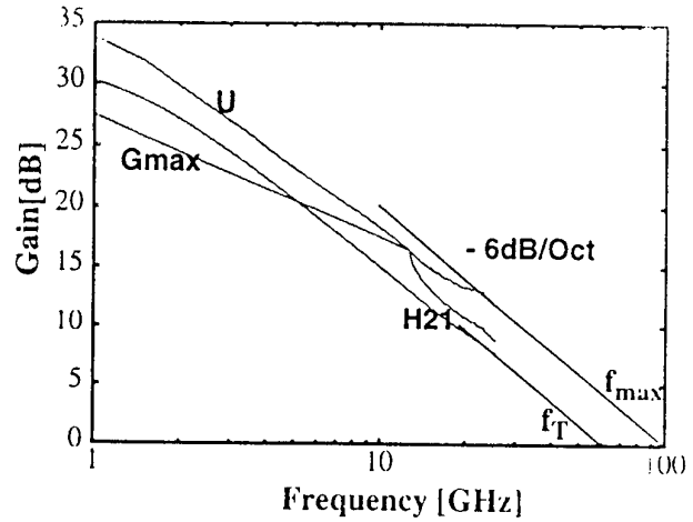
Fig. 2: High-frequency performance of 2 \times 30 \mu\text{m} HBT at V_{CE} = 3\text{V} and I_C = 20\text{mA}
