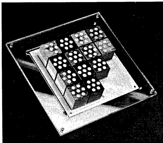
Figure 5 : Concept of 3D-Module Ka band Active Antenna
