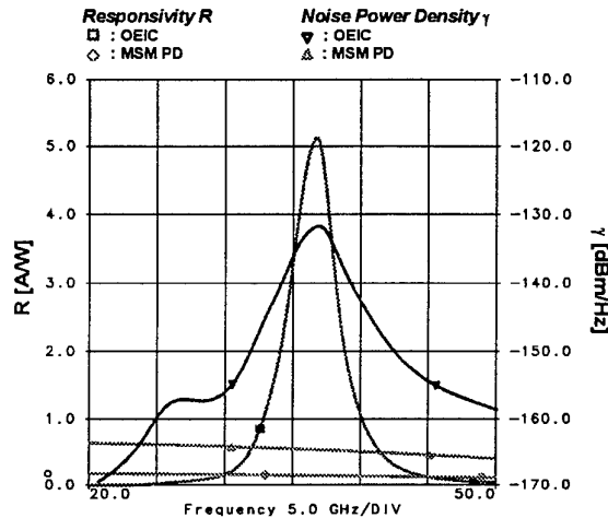
Fig. 4: Simulated frequency response of MSM PD and OEIC
