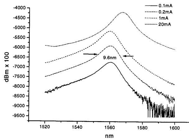
Figure 3: Spectra for different currents
