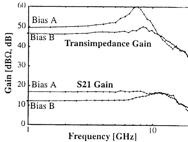
Fig. 4 Transimpedance and S_{21} gain of the cascode amplifier under different bias conditions
