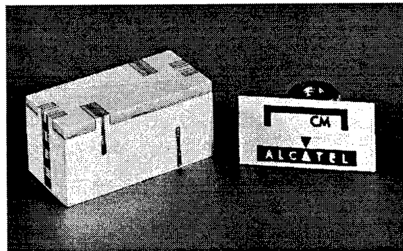
Figure 4 : Measured gain response (left) and photograph of the realized 3D module.
