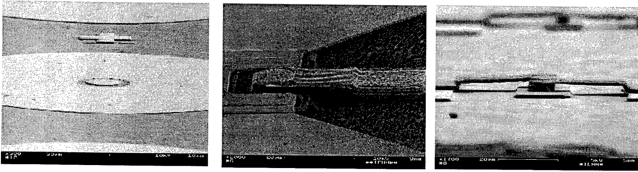
(a) (b) (c) Fig. 1: SEM views of coaxial-type (a), coplanar waveguide type (b) and series type (c) test patterns.
