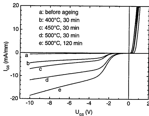
Fig. 4: Gate diode I/V characteristics of a GaN-HFET before and after ageing.
