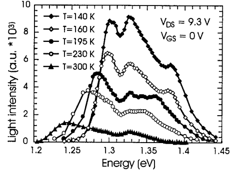
Fig.4 High resolution analyses of the channel recombination peak measured at different measured at different ambient temperatures.
