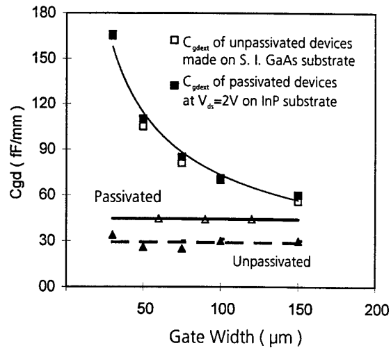
Fig. 4: Comparison of the extracted C_{gd} on 0.15 \mu\text{m} HEMTs on InP and semi-insulating GaAs substrates. The effect of silicone nitride on the intrinsic C_{gd} is shown.
