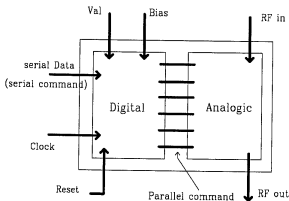
Figure 7 : Schematic of Mixed RF / Digital control function.
