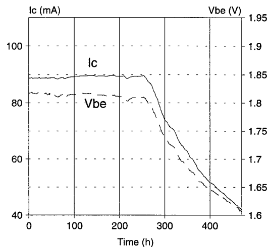
Fig.4 Life time measurements of a 3 \times 15 \mu\text{m}^2 HBT at a collector current density of 2 \times 10^5 \text{ A/cm}^2
