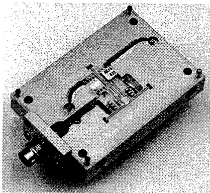
Fig. 2: W-band wave guide module of 94 GHz dual channel heterodyne receiver.
