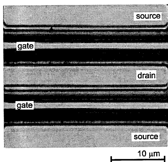
Fig. 1: Microscope image of a GaN MESFET device with Ti/WSiN ohmic contacts for source and drain.
