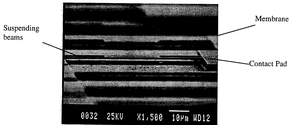
Figure 2: SEM micrograph of a freestanding movable membrane suspended by 4 beams.
