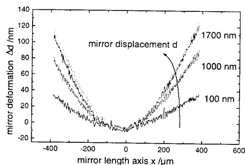
Fig. 3: Actuation induced deformation of thermal actuated mirror
