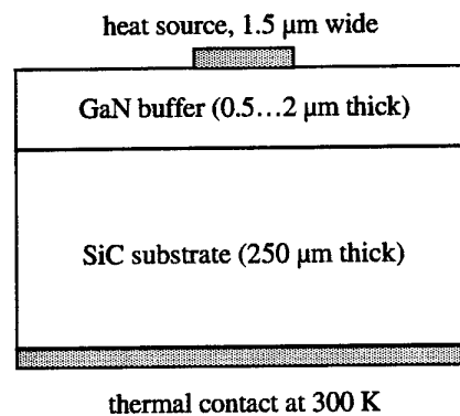
Fig. 2: simulated geometry
