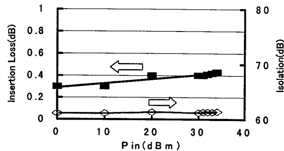
Fig.4 Power transfer characteristics of the developed IC at 1GHz
