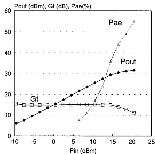
Fig.3 Output power P_{\text{out}} , power added efficiency P_{\text{ae}} and power gain G_t against input power P_{\text{in}} , measured at 2 GHz for a 10 \times 3 \times 30 \mu\text{m}^2 power HBT ( V_{\text{CE}} = 4.5 \text{ V} )
