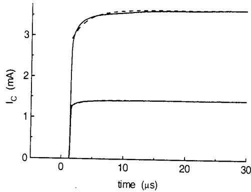
Figure 2 – Collector current transients for base biases of 1.390 and 1.425V. The solid lines show experimental results, and the dashed lines the fit.
