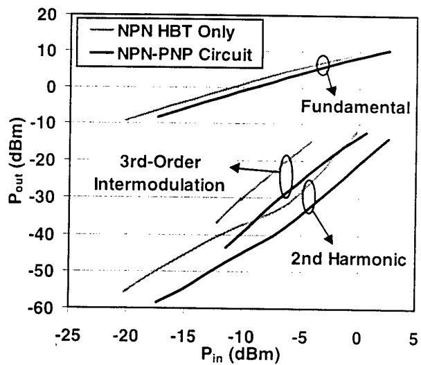
Figure 4: Power characterization of NPN/PNP push-pull common-emitter amplifier at 8 \text{ GHz} . The 2^{\text{nd}} harmonic and 3^{\text{rd}} -order intermodulation ( 500 \text{ kHz} separation) are improved when compared to a single NPN HBT amplifier.
