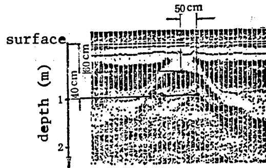
Figure 6. Double-Target Test
