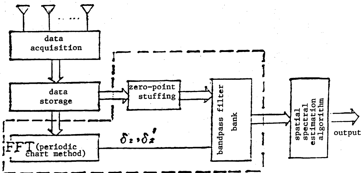
Figure 1. Schematic of Spatial Filter Preprocessing Implementation
