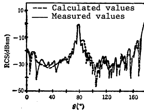
Figure 3. Radar Cross Section of a Cone (horizontal polarization, monostatic setup)
