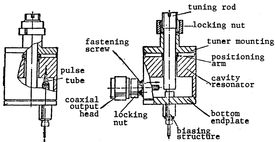
Figure 1. Oscillator Structure
