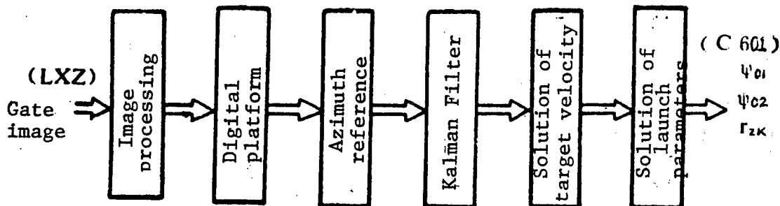
Figure 8. Computational Flow Diagram of the Fire Control Unit
