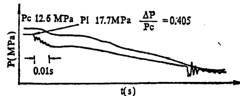
Figure 10. Slow Extinguishment Process (DB, water + 0.5% CE)
